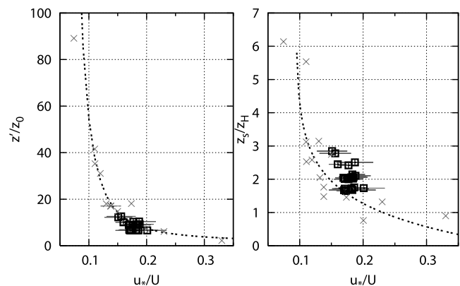
Figure 12. Variation of u^*/U for neutral conditions with nondimensional heights (left) z/z_0 and (right) z_s/z_H . Mean and standard deviation are shown for a normalized height and direction data. Line in left panel is based on log profile, and line in right panel is based on Roth [2000, equation (5)] ( u^*/U = 0.094 + 0.353 \exp[-0.946(z_s/z_H)] ). Squares are data from this study, and crosses are data reported by Roth [2000, Figure 1]. See color version of this figure in the HTML.
