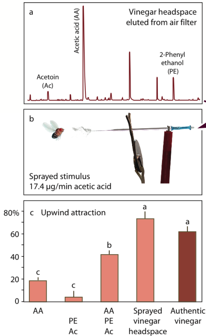
Fig. 1 Attraction of 2-d-old starved Drosophila melanogaster adults in a wind tunnel to GC-MS analyzed (a) and defined odor samples that were released from a glass capillary attached to a piezo-ceramic disk (piezoelectric sprayer) (b). The release rates of acetic acid (AA), the main vinegar compound (17.4 µg/min), ethyl acetate (0.103 µg/min), acetoin (Ac; 0.58 µg/min) and 2-phenyl ethanol (PE; 1.22 µg/min) in sprayed headspace and in synthetic blends mimic vinegar headspace. Flies were attracted to sprayed synthetic vinegar compounds, sprayed vinegar headspace extracted from air filters and to authentic vinegar headspace from a wash bottle (c). Different lowercase letters in (c) indicate significant differences according to ANOVA followed by Tukey's test ( N=5 batches of 20 flies; F=50.61 ; df=24 , P<0.001 ; error bars show standard deviation of the mean).
