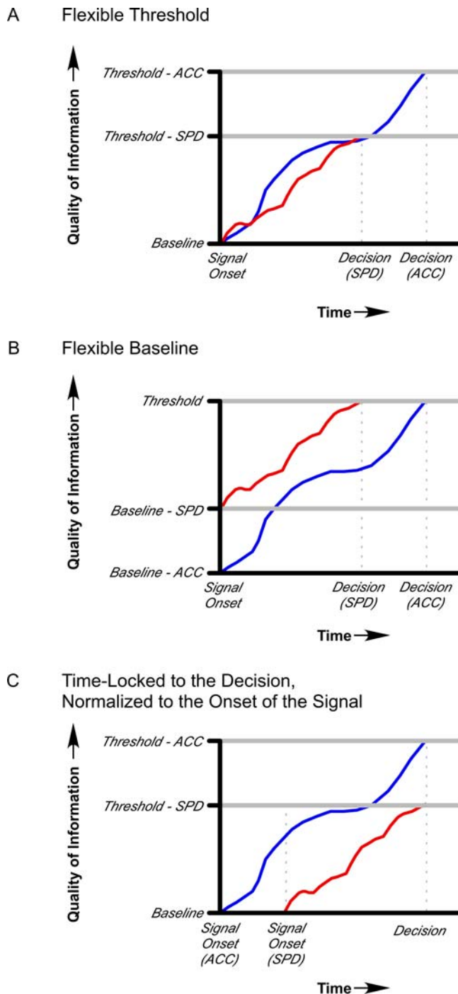
Figure 1. An illustration of a simple accumulator model of the speed-accuracy tradeoff (SAT). According to this type of model, task-relevant evidence (e.g. motion coherence) accumulates over time from a starting point until a threshold for decision is reached (horizontal grey bars). The vertical stippled lines mark the time, along the x-axis, when a response would be made. (a) In a flexible threshold account of the SAT, emphasizing the speed (SPD) of responding lowers the threshold for decision-making relative to emphasizing accuracy (ACC) of responding, thus reducing the amount of accumulated evidence (and time) prior to the response. (b) In a flexible baseline account of the SAT, emphasizing the speed of responding would increase the baseline level of activity towards a decision threshold, thereby reducing the amount of evidence, and hence the time, that is required to reach that threshold. These two models are not necessarily mutually exclusive. (c) If the accumulation functions are aligned to the time that the decision is
