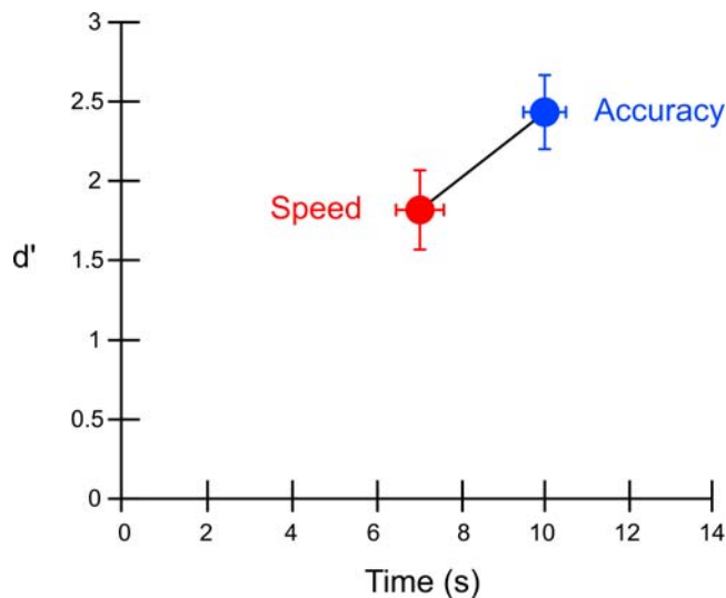
Figure 3. Sensitivity to detect coherent motion ( d' ) versus response time (s) as a function of Speed and Accuracy instructions.
