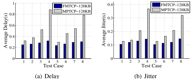
Fig. 12: The average delivery delay and jitter of blocks of FMTCP and IETF-MPTCP. The parameters of the subflow 1 remain the same (100ms delay, 0.1% packet loss). The delay and loss rate of the subflow 2 are shown in Table II.
