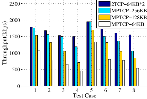
Fig. 2: Goodput comparison between IETF-MPTCP and 2-TCP
