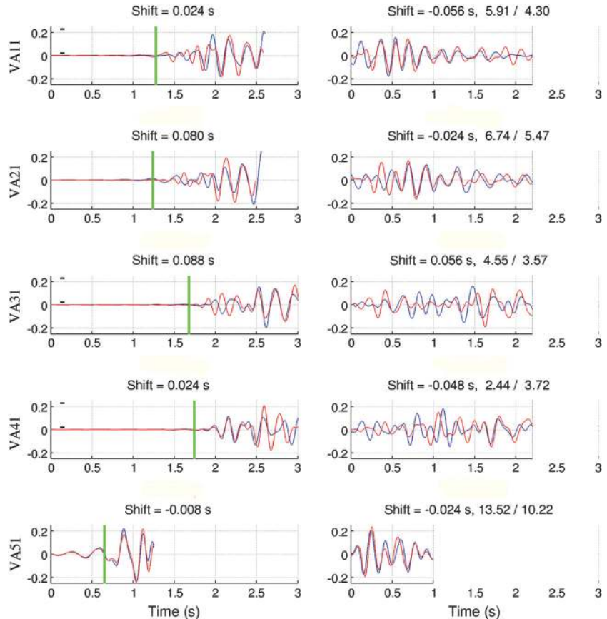
Figure 7. Comparisons between modeled waveforms (red) and synthetic data (blue) at five stations with perturbed velocity model. From top to bottom, waveforms from the vertical components at stations one through five, respectively, are shown. The waveforms are filtered between 3 and 9 Hz. The left column shows P-waves and right column shows S-waves. The green lines indicate the first P-arrival times. For P-waves, zero time means the origin time, and for S-waves, zero time means the S-wave arrival time predicted by the calculated traveltimes. The “shift” in the title of each subplot indicates the time shifted in the data to align with the synthetic waveforms. In the left column, the + or - signs indicate the first-arrival polarities of P-waves in the synthetic data and those in the modeled data, respectively. In the right column, the number to the left of the slash denotes the S/P amplitude ratio for the synthetic data, and the number to the right of the slash denotes the ratio for the modeled waveform.
