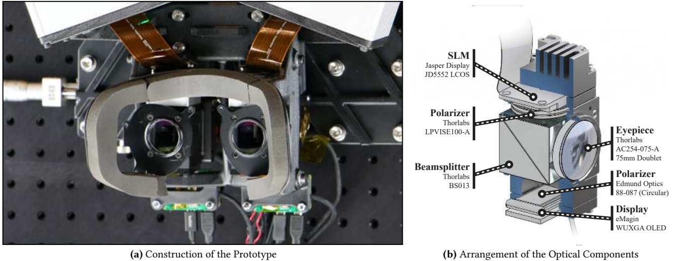
Fig. 10. Our binocular focal surface display prototype incorporates commodity optical and mechanical components, as well as 3D-printed support brackets. (a) The prototype is mounted to an optical breadboard to support the comparatively large LCOS driver electronics. A chin rest is used to position the viewer within the eye box. (b) A cutaway of the prototype exposes the arrangement of the optical components.
