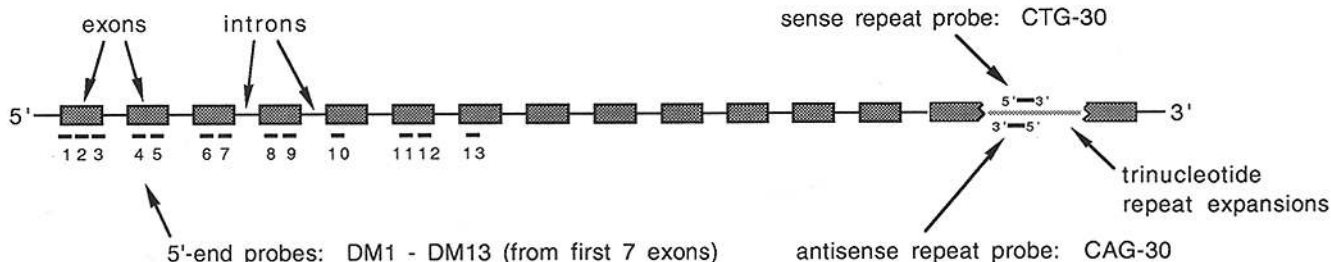
Figure 1. Schematic diagram showing the probes that were used to detect the myotonic dystrophy gene and its transcripts.
