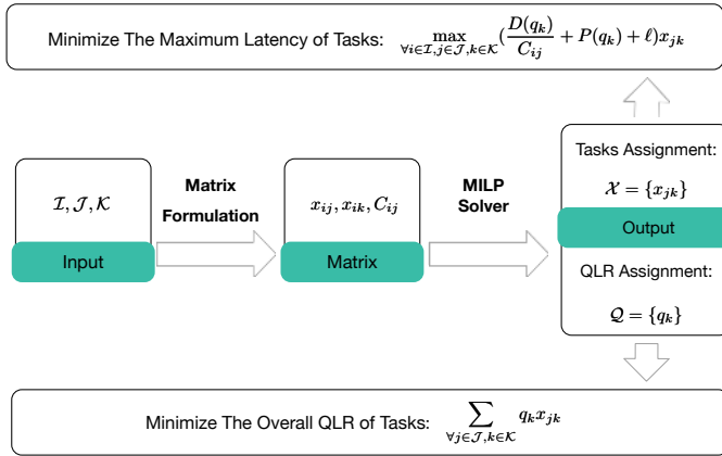
Fig. 2: Workflow of MBO
