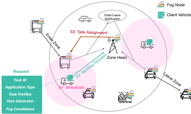
Fig. 1: Overview of Folo. A light magenta circle represents the communication range of the client vehicle in the center. Here the communication is limited to one hop for DSRC.
