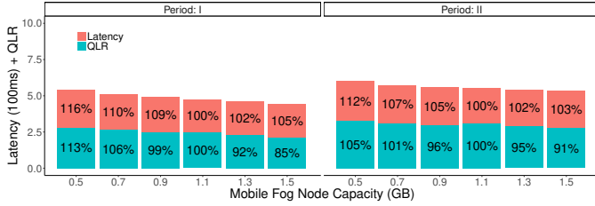
Fig. 8: Performance vs. Memory Capacity
