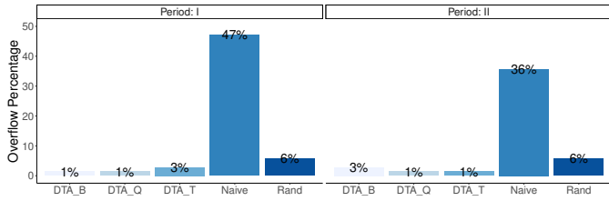
Fig. 9: Server Memory Overflow
