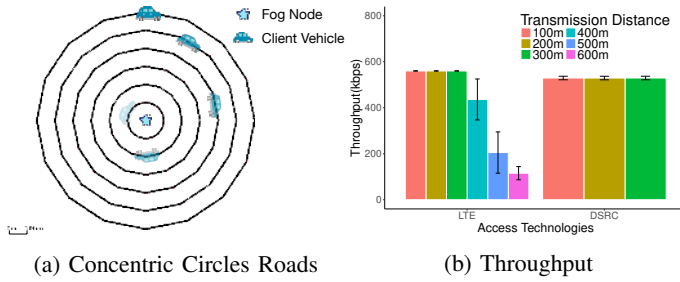
Fig. 4: Network performance of LTE vs. DSRC
