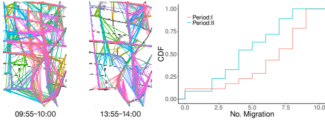
(a) Visualization of taxi traces (b) Mobility-related task migration
