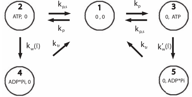
FIG. 2. The two-motor model with a power stroke is schematically depicted with transitions between the five chemical states. The chemical states (0,0) , (\text{ATP},0) , (0,\text{ATP}) , (\text{ADP}^*\text{Pi},0) , and (0,\text{ADP}^*\text{Pi}) are numbered from 1 to 5, respectively. The rate k_w(\ell) [or k'_w(\ell) ] is the length-dependent transition rate from the (\text{ATP},0) [or (0,\text{ATP}) ] state to the active translocation state (\text{ADP}^*\text{Pi},0) [or (0,\text{ADP}^*\text{Pi}) ]. The rate k_{tr} , assumed to be length independent, is the transition rate from the active translocation state (\text{ADP}^*\text{Pi},0) or (0,\text{ADP}^*\text{Pi}) to the apo state (0,0) . The rate k_p is the ATP binding rate from the (0,0) to the (\text{ATP},0) [or (0,\text{ATP}) ] state. Finally, the rate k_{p,s} is the transition rate which makes ATP sampling possible; it is the ATP unbinding rate of the left (or right) motor to the apo state, with the possibility of subsequent binding to the right (or left) motor.
