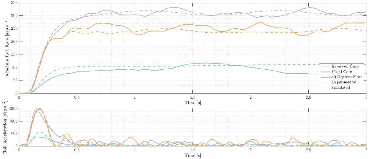
Fig. 9 Example experimental and numerical time traces for the removed, fixed, and free30 configuration at 25 \text{ m s}^{-1} and aileron angle of 14 degrees
