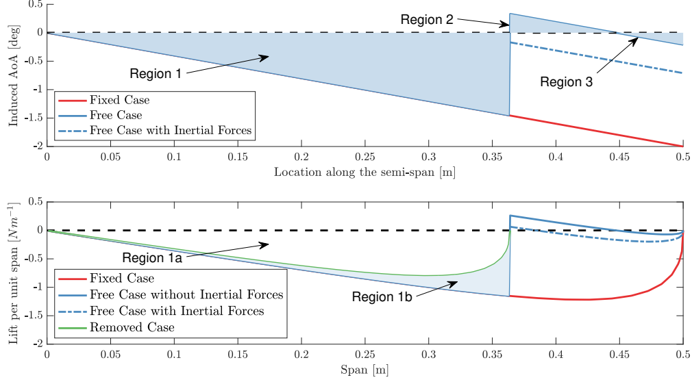
Fig. 12 A diagrammatic representation of the aerodynamic and inertial forces acting on the fixed, free and removed case due to a rolling motion of 60 \text{ deg s}^{-1}
