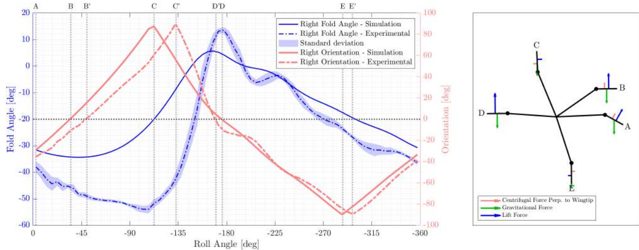
Fig. 17 On the left, the simulated and experimental variation of the fold angle and absolute orientation of the right wingtip during the steady roll rate region for a flare angle of 10 degrees, aileron angle of 14 degrees and a velocity of 20 \text{ m s}^{-1} . On the right, the position of the right wingtip at locations A thru E.
