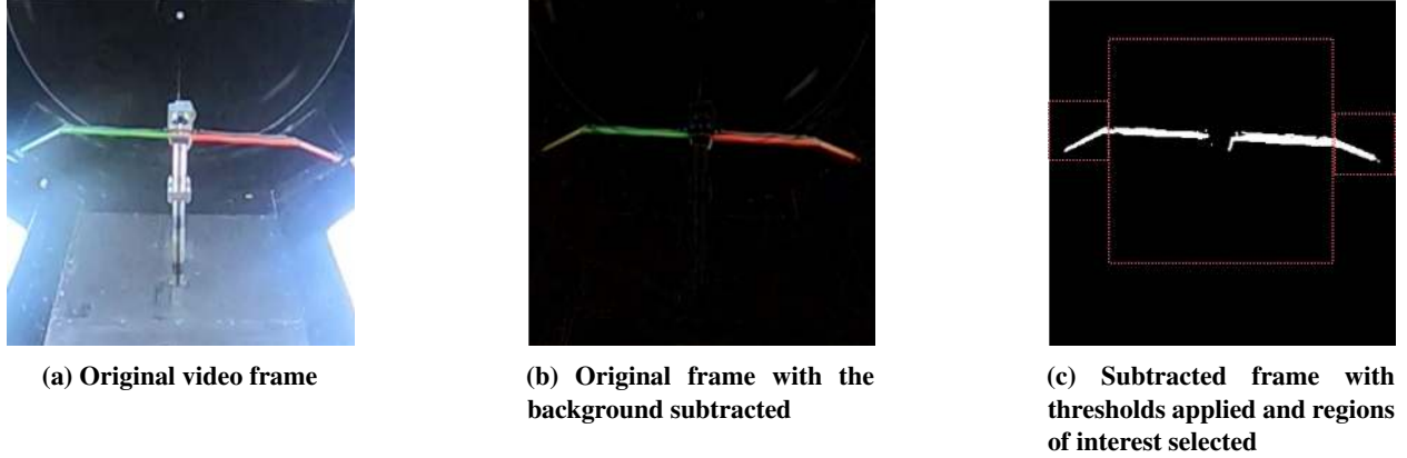
Fig. 4 An overview of the computer vision algorithm used to measure the roll and fold angles of the wind tunnel model
