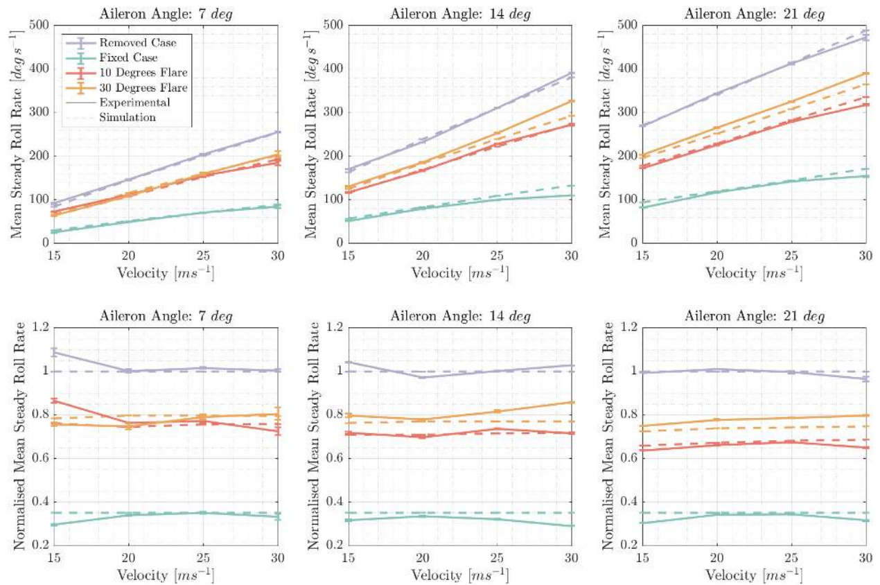
Fig. 10 Mean steady roll rates at each aileron angle and velocity for each model configuration. In the bottom row values have been normalised by that of the simulated removed case at each velocity
