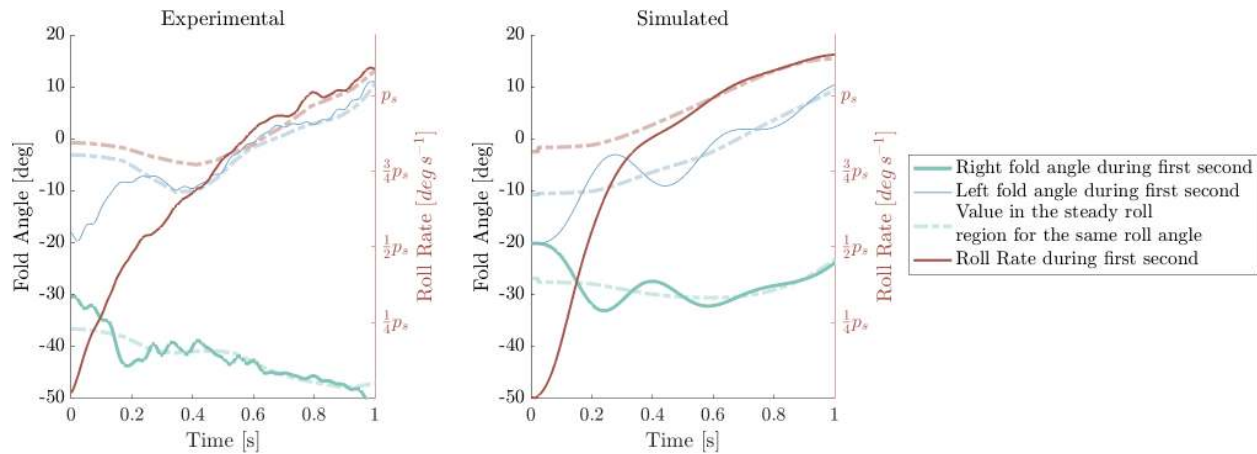
Fig. 24 A comparison of the simulated and experimental response in the roll acceleration region of the left and right wingtip with a flare angle of 10 degrees, at a velocity of 20 \text{ m s}^{-1} and an aileron angle of 7 degrees
