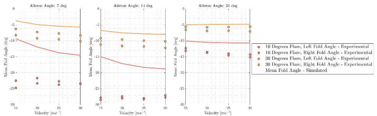
Fig. 11 The mean fold angle of each wingtip at each aileron angle and velocity for each model configuration
