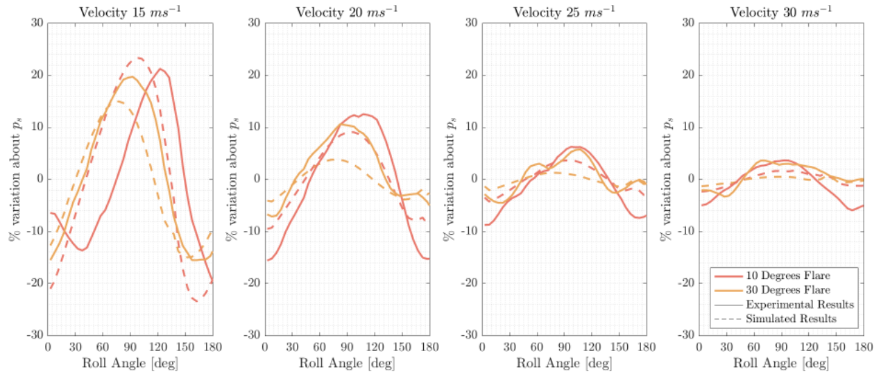
Fig. 14 Variation with roll of the roll rate as a percentage of the steady roll rate, for each configuration at multiple velocities and an aileron angle of 14 degrees
