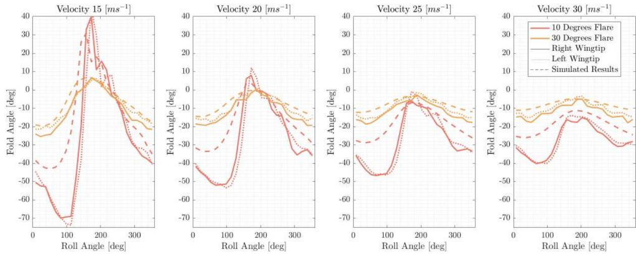
Fig. 18 Variation of the left and right fold angle with roll, for each configuration at multiple velocities and an aileron angle of 14 degrees
