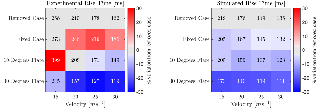
Fig. 22 A comparison of the average time constant for each configuration at each velocity, across all aileron angles
