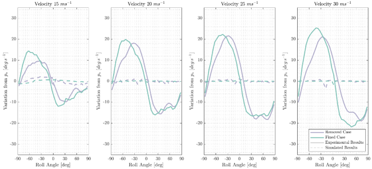
Fig. 13 Variation from the steady roll rate with roll, for each configuration at multiple velocities and an aileron angle of 7 degrees
