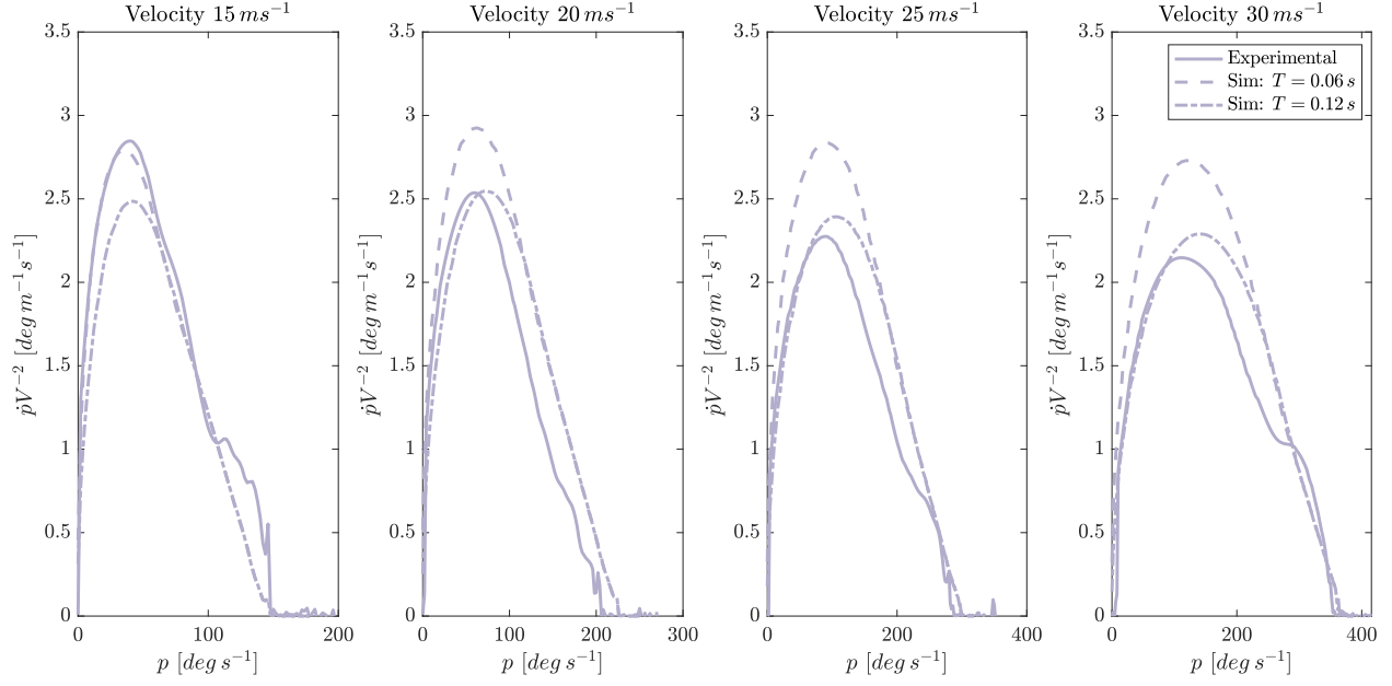
Fig. 20 A comparison of the experimental and simulated acceleration, velocity phase space for the removed case.
