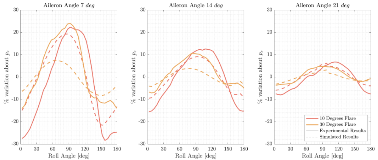
Fig. 15 Variation with roll of the roll rate as a percentage of the steady roll rate, for each configuration at multiple aileron angles and a velocity of 20 ms^{-1}
