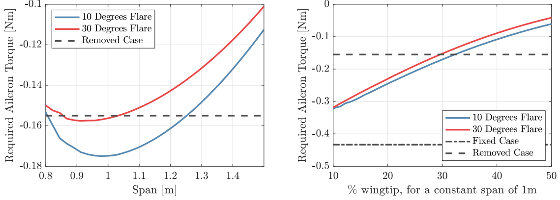
Fig. 25 The variation in the required aileron torque to maintain a roll rate of 60 \text{ deg s}^{-1} at zero roll angle and an airspeed of 25 \text{ m s}^{-1} as a function of a) span, with the hinge line at 728 mm b) Sigma - The ratio of the total span that is folding wingtip, for a constant total span of 1m
