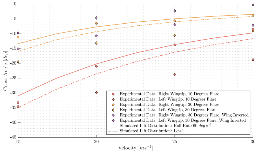
Fig. 8 The coast angle of each wingtip with flow speed, for each model configuration
