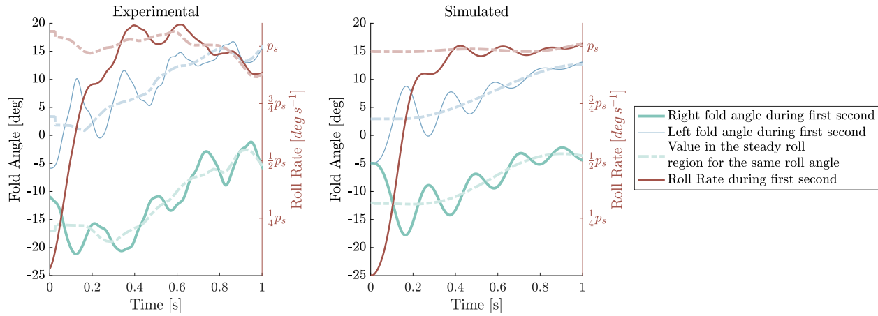
Fig. 23 A comparison of the simulated and experimental response in the roll acceleration region of the left and right wingtip with a flare angle of 30 degrees, at a velocity of 25 \text{ m s}^{-1} and an aileron angle of 14 degrees
