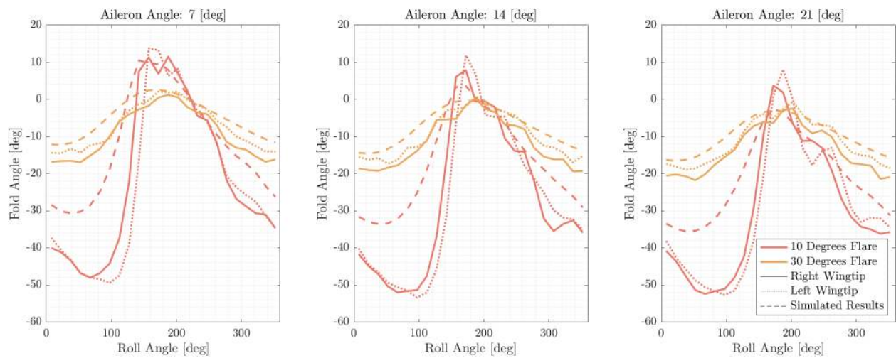
Fig. 19 Variation of the left and right fold angle with roll, for each configuration at multiple aileron angles and a velocity of 20 m s^{-1}
