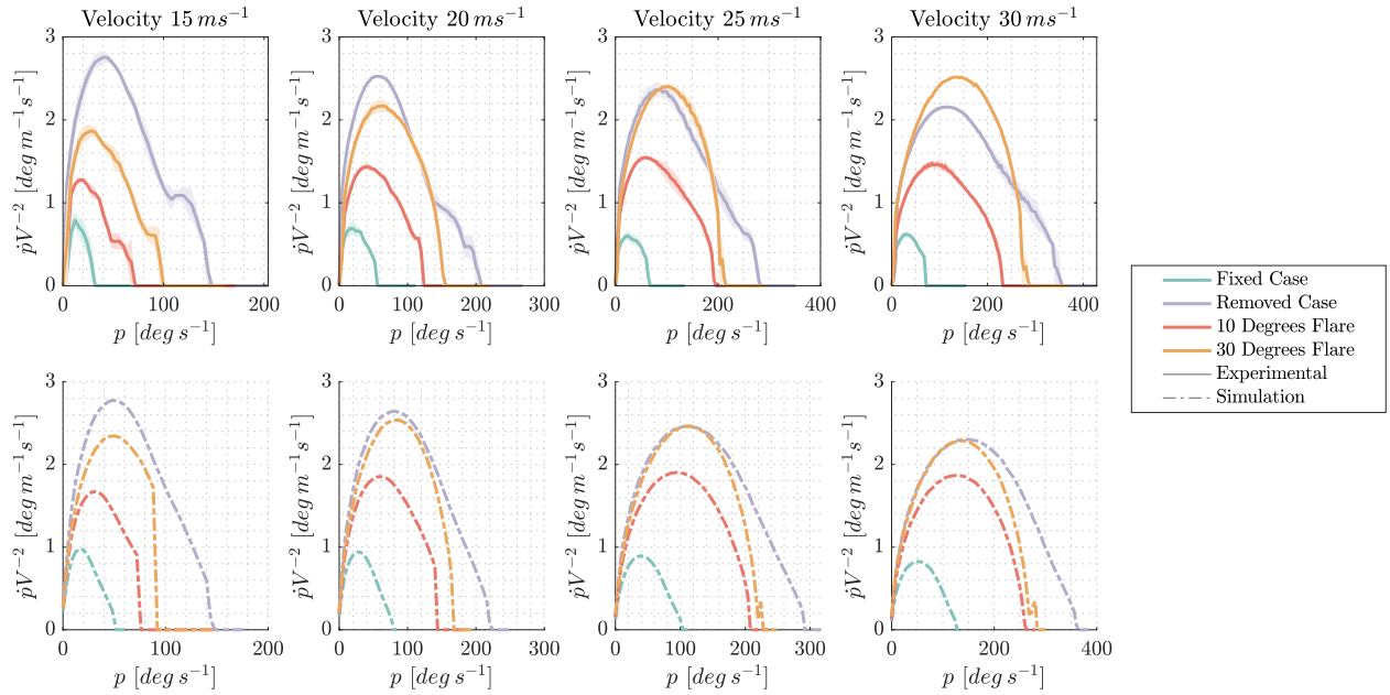
Fig. 21 A comparison of the experimental and simulated acceleration, velocity phase space for each configuration
