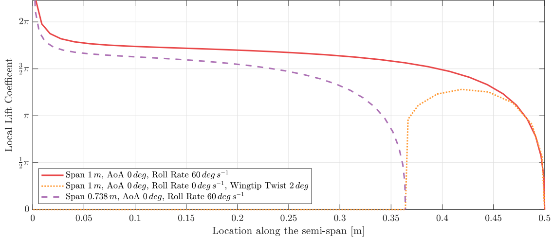
Fig. 6 A comparison of the three lift distributions used in the simulated results
