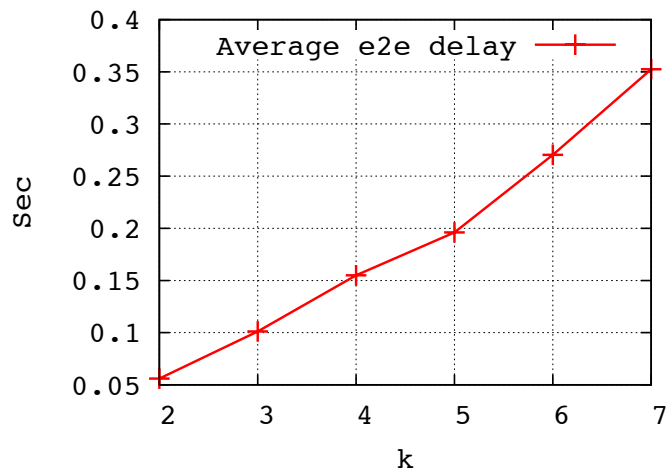
Fig. 11. Average latency
