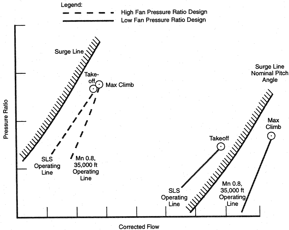
Figure 14. ADP Has Inadequate Surge Margin With Fixed Geometry Fan
