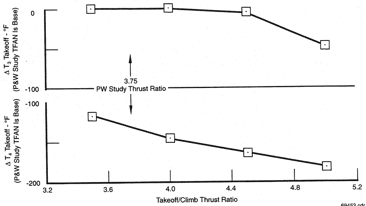
Figure 19. Airplane Thrust Requirements Impact Rating Differences
