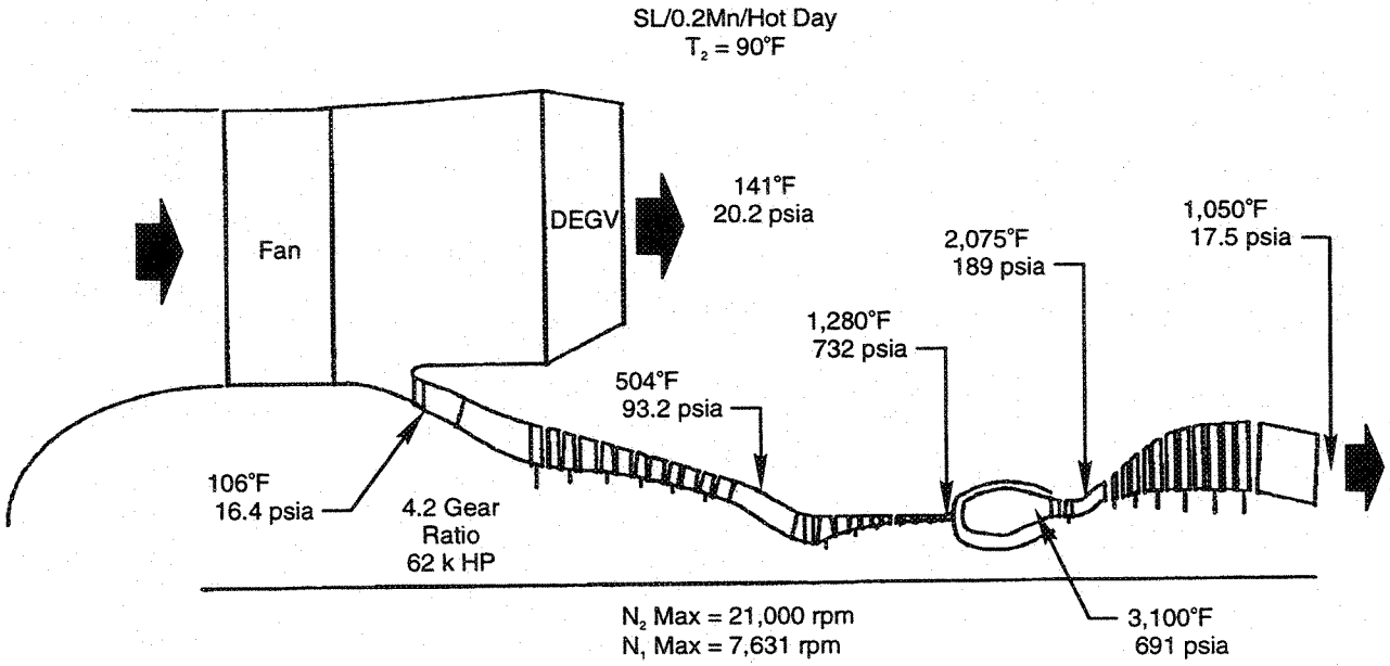
Figure 3. 2005 EIS ADP Maximum Temperatures and Pressures
