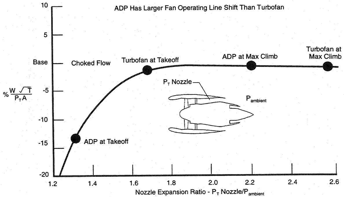
Figure 13. Lower Fan Pressure Ratio ADP Nozzle Unchokes More at Takeoff
