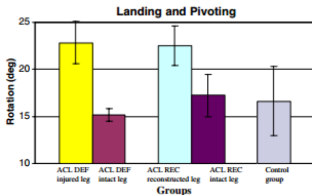
FIGURE 4. Group mean and SD values for maximum range of motion of the tibial internal–external rotation during the pivoting period for the landing and pivoting activity.
