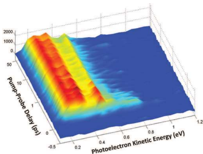
FIG. 6. Time-resolved photoelectron spectrum of indole following 249 nm excitation and subsequent ionisation with a 300 nm probe. For clarity, the time dependence is plotted using a linear scale in the region -0.5 – 0.5 ps and a logarithmic scale for delay times between 0.5 and 50 ps.
