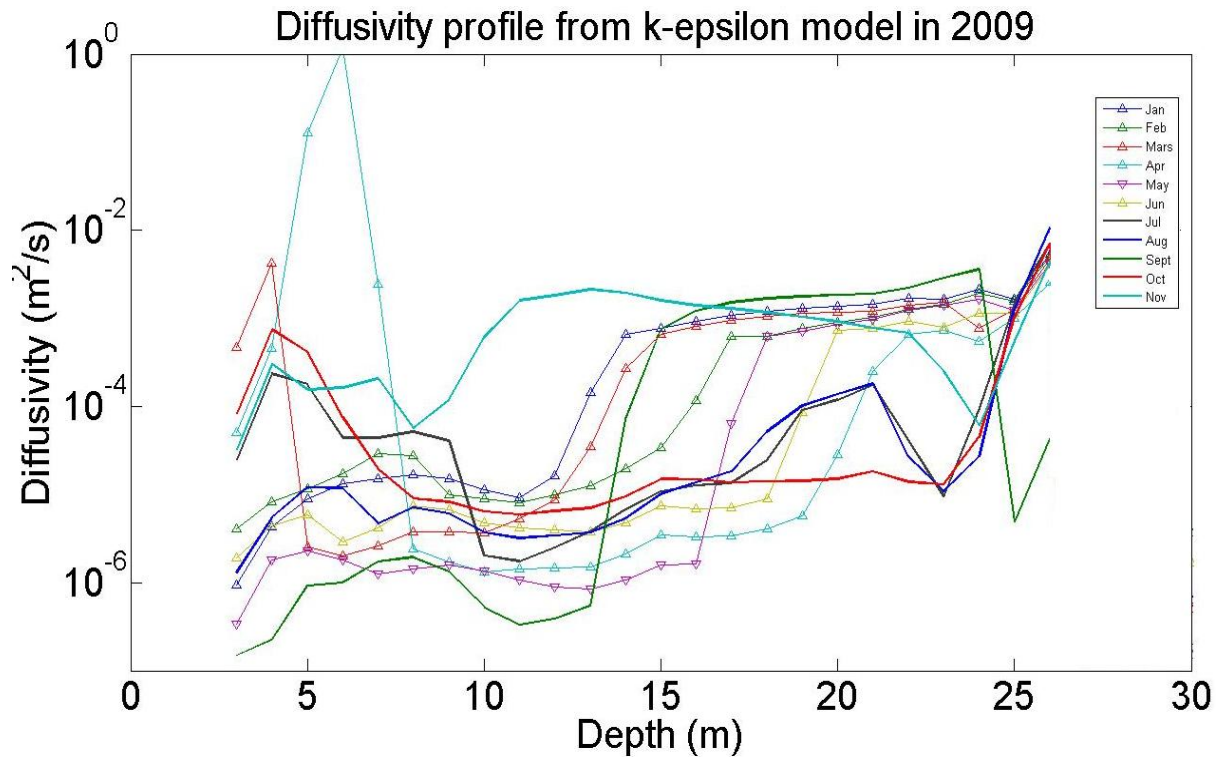
Appendix 7. The resulting time series of vertical turbulent diffusivity obtained from the physical k-epsilon model
