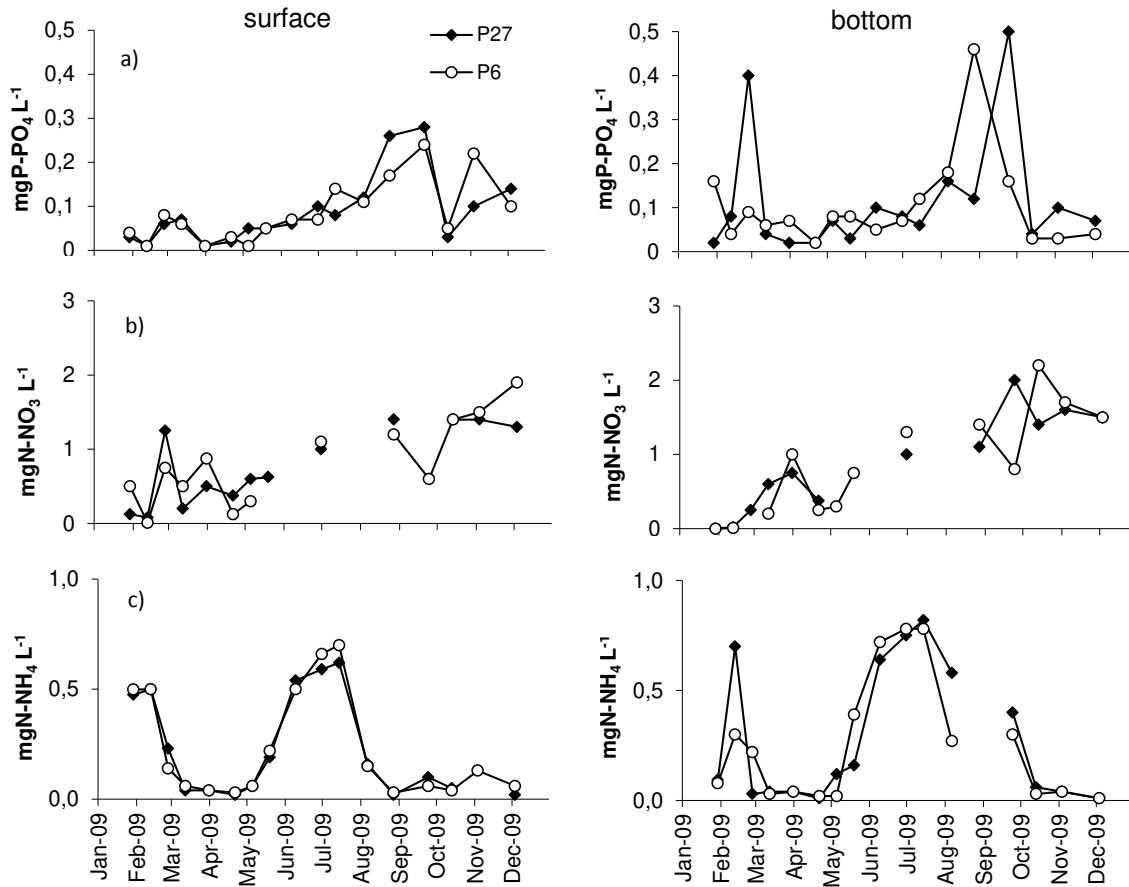
Figure 7: Comparison of the seasonal variations in a) P-PO_4^{3-} , b) N-NO_3^- , and c) N-NH_4^+ in the water column at the two sampling points P6 and P27 (surface and bottom) in the Cointzio reservoir.
