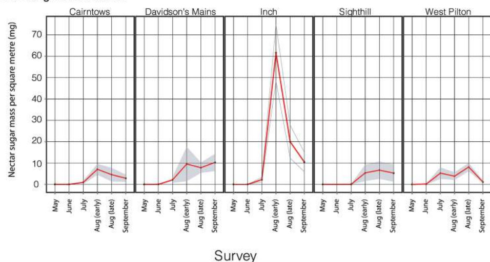
Fig 4. Seasonal patterns in daily nectar sugar availability for individual Edinburgh meadows sown with A. perennial, B. annual A1, and C. annual A2 treatments. Data were sampled at three-week intervals through 2013. Values at each time point are means based on 20x 1m 2 quadrats, with dark shading showing 95% confidence limits. The poor performance of the Saughton perennial meadow was due to accidental mowing, and this replicate was excluded from statistical analyses.
