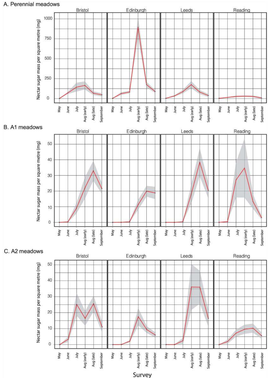
Fig 6. Seasonal patterns in nectar sugar availability across four UK cities for meadows sown with A. perennial, B. annual A1, and C. annual A2 treatments, assessed at three-week intervals in 2013. Values at each time point are means based on 7x 1m 2 quadrats, with dark shading showing 95% confidence limits. Plots for individual sites are shown for Bristol, Reading and Leeds in S3 Fig .
