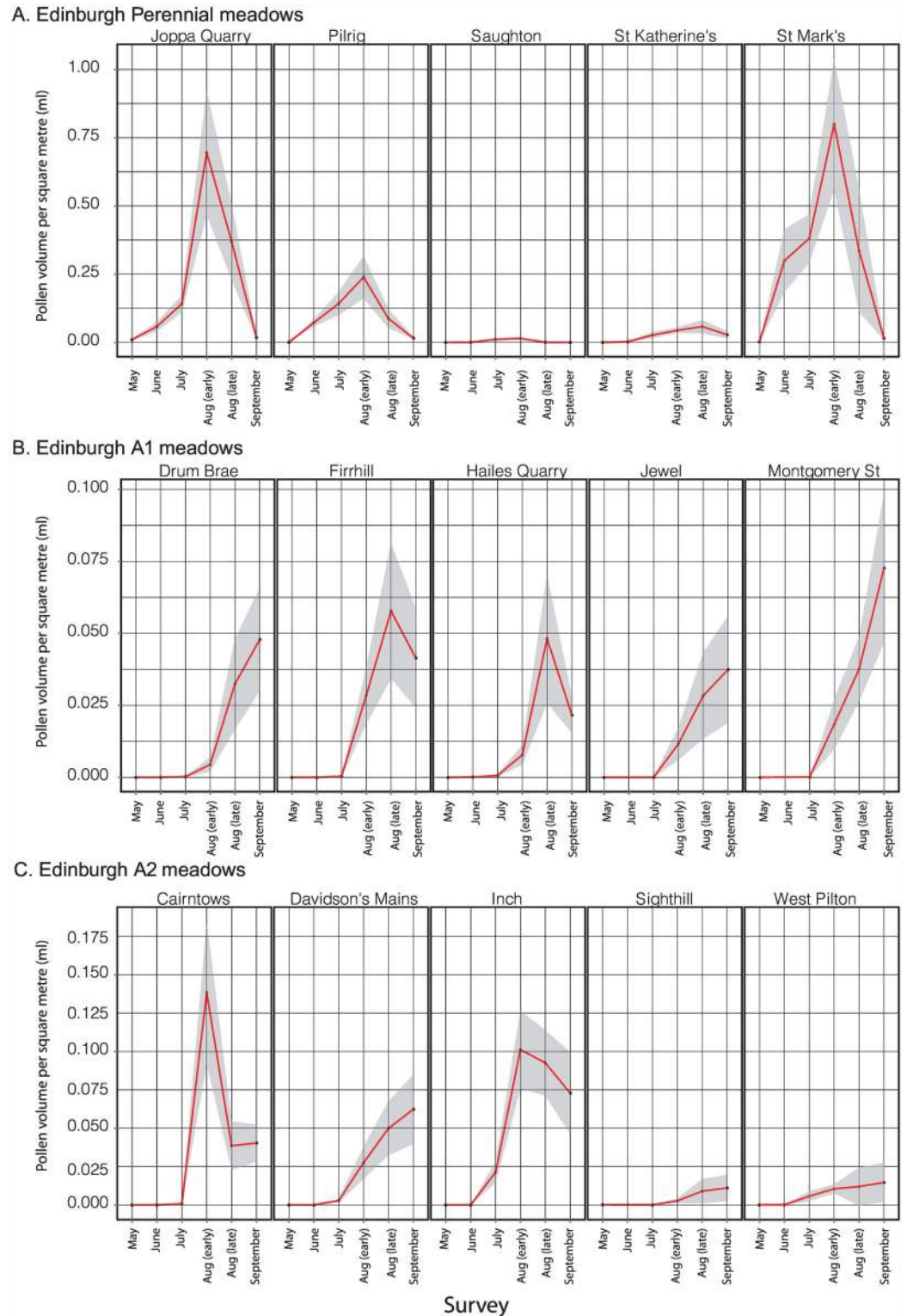
Fig 7. Seasonal patterns in daily pollen availability for individual Edinburgh meadows sown with A. perennial, B. annual A1, and C. annual A2 treatments. Data were sampled at three-week intervals through 2013. Values each time point are means based on 20x 1m 2 quadrats, with dark shading showing 95% confidence limits.
