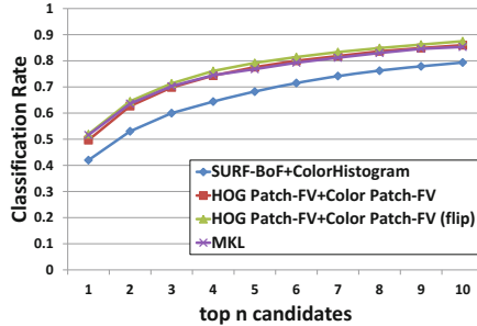
Fig. 2. Classification rate by proposed method, client side[6] and server side[1]
