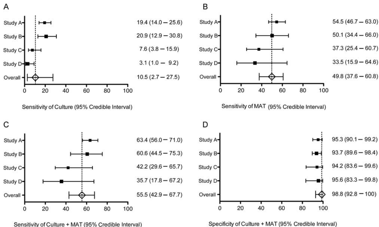
Figure 3. Forest plot of sensitivity and specificity of culture ( A ), microagglutination test (MAT; B ), and the combination of culture and MAT (culture + MAT; C and D ) for leptospirosis estimated by Bayesian latent class models (LCMs) and random-effects meta-analysis models. Squares represent median estimates of the sensitivities and the specificities, and the size of the square represents the size of the study. Horizontal lines represent 95% credible intervals of the estimates. Bayesian LCM assuming conditional dependence between culture and PCR and between MAT and lateral flow (LF) was used for study A, and Bayesian LCM assuming conditional dependence between MAT and immunofluorescence assay was used for study B. Bayesian LCM assuming conditional independence between tests and consistency of test accuracies between study sites was used for studies C and D. Meta-analysis was performed by application of random-effects variables into the combined data set of all 4 studies, assuming conditional dependence between culture and PCR, between MAT and LF, and between MAT and IFA. Abbreviations: IFA, immunofluorescence assay; LCM, latent class model; LF, lateral flow; MAT, microagglutination test; PCR, polymerase chain reaction.
