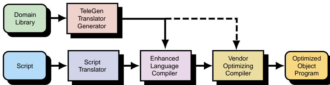
Figure 2: Telescoping Languages
