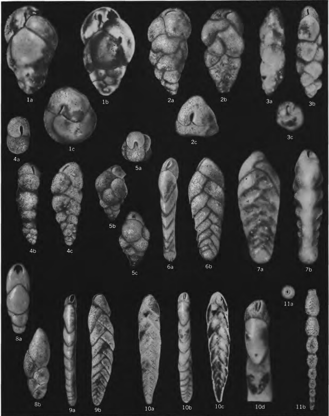
BULIMINA, NEOBULIMINA, BOLIVINA, LOXOSTOMA, PLEUROSATOMELLA, AND STILOSTOMELLA
