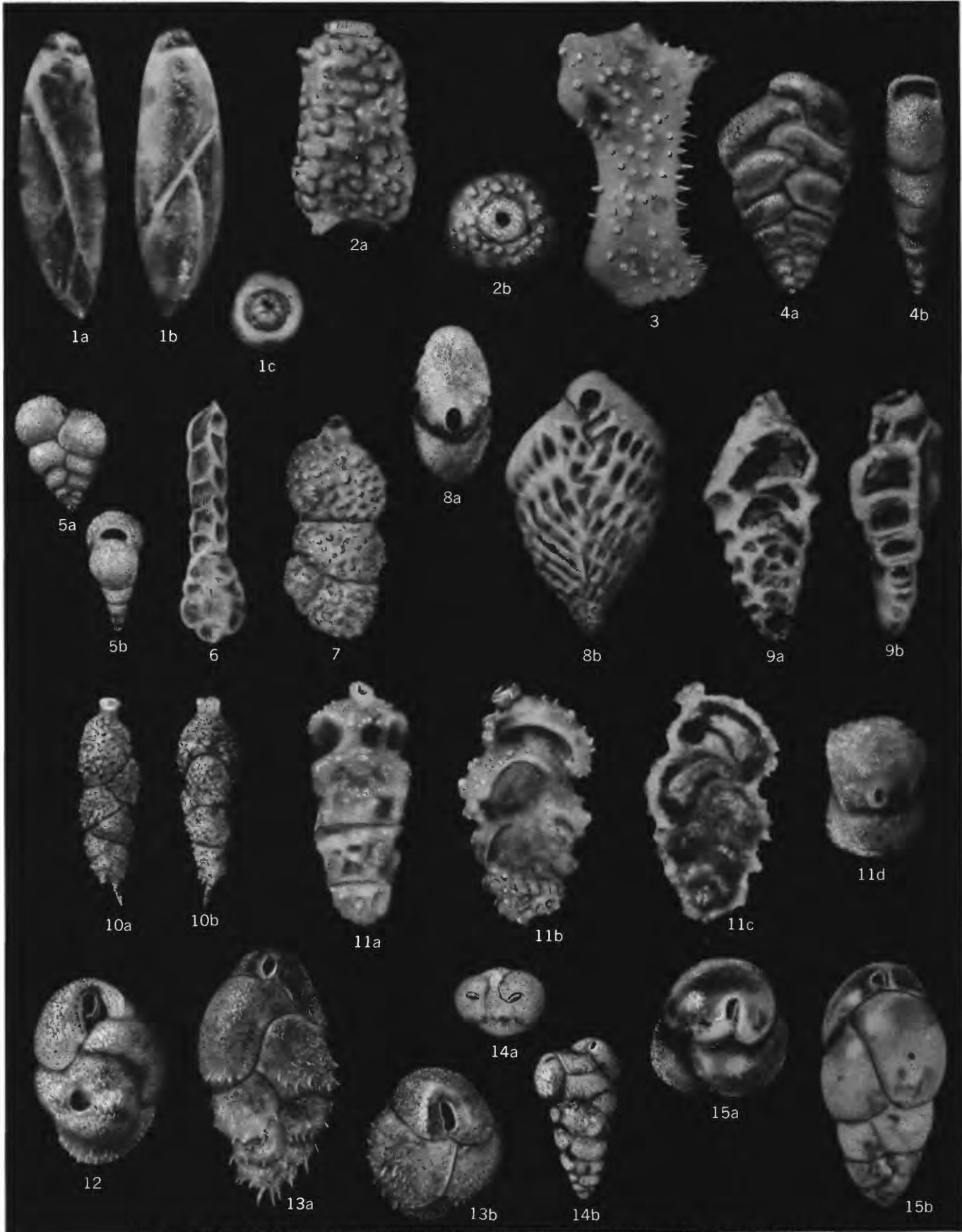
PYRULINA, RAMULINA, HETEROHELIX, BOLIVINOPSIS, RECTOGUEMBELINA, BOLIVINOIDES, TAPPANINA, EOUVIGERINA, AND BULIMINA
