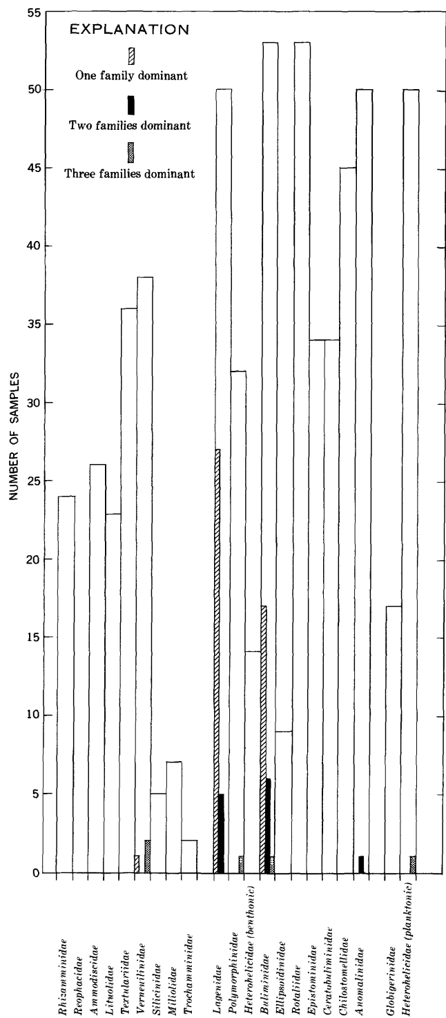
FIGURE 11.—Distribution of families in 53 samples containing 11 or more species from the calcareous biofacies. See figure 9 for explanation.
