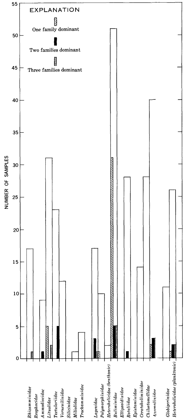
FIGURE 10.—Distribution of families in 66 fossiliferous samples containing one to 10 species from the calcareous biofacies. See figure 9 for explanation.
