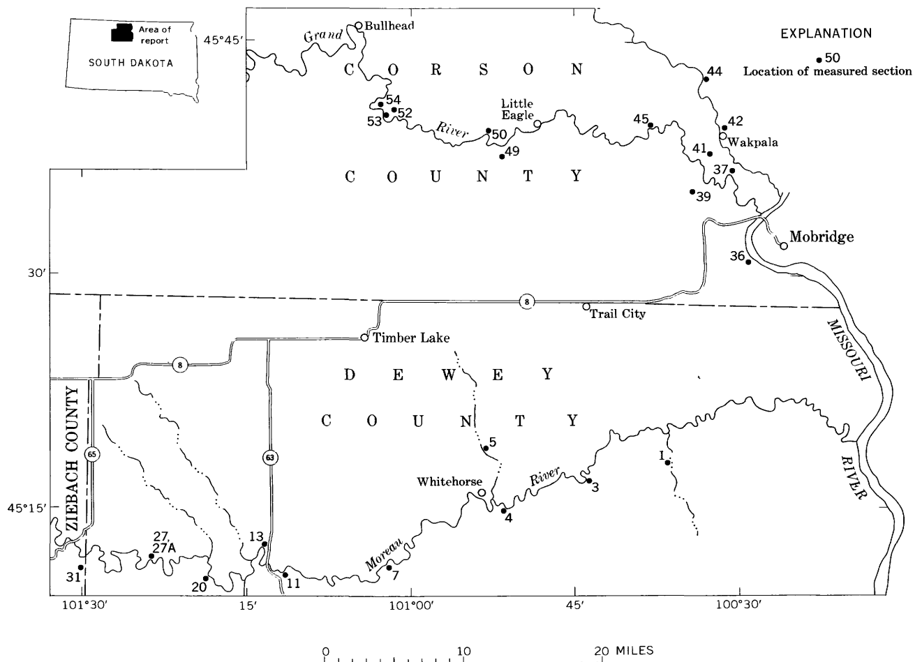
FIGURE 1.—Index map of north-central South Dakota showing approximate locations of measured sections. Location numbers shown here match section numbers shown on plate 12 and in figures 4 and 5.
