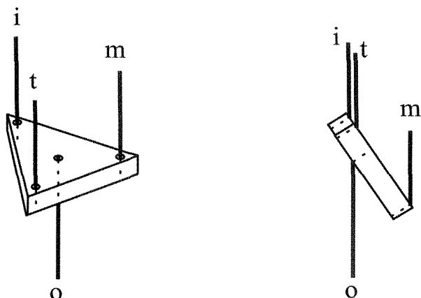
Figure 5. Triangle distributing the operating force from the operating cable (o) to the thumb tendon (t), the index tendon (i) and the middle finger tendon (m). Left: holding a large object; right: holding a small object between the thumb and the index finger only.
