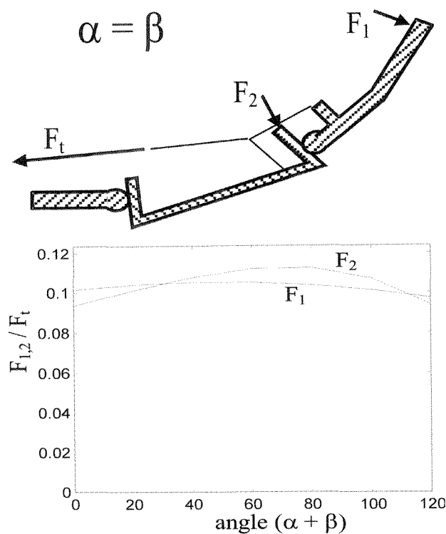
Figure 4a. Force transmission ratio as a function of \alpha + \beta .
