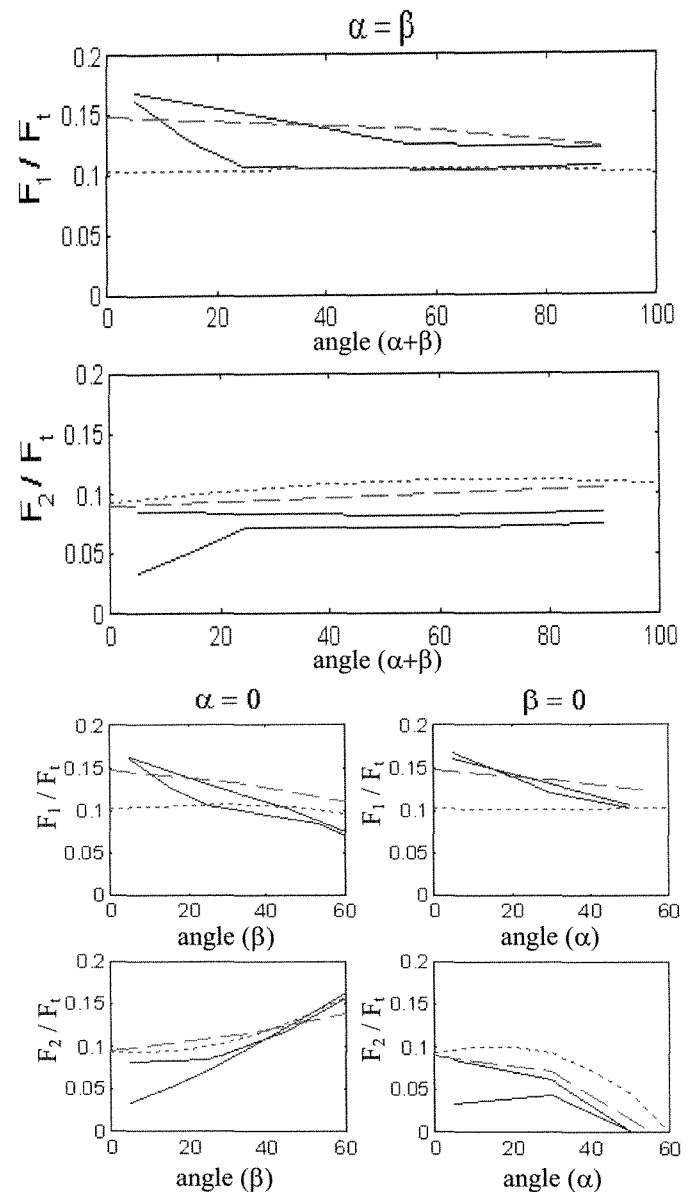
Figure 9. Force transmission ratios as a function of finger position. The dotted lines are the theoretical values as in Figure 4 . The dashed lines are the measurements done on the mechanism without the glove and the compensation springs; the solid lines are the maximum and minimum measurements with the glove present. Top two figures: the transfer ratios in the situation for which the design was optimized ( \alpha = \beta ). Bottom four figures: the ratios in the extreme situations: \alpha = 0 (left figures); \beta = 0 (right figures).
