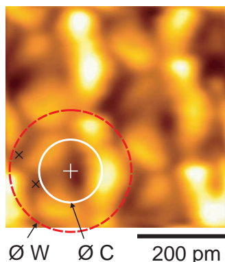
Fig. 4. Magnified view of Fig. 2F, demonstrating a lateral resolution of 77 pm (distance between the black crosses). The solid circle has a diameter of 142 pm, indicating the diameter of a carbon atom. The dashed circle shows the diameter of a tungsten atom (274 pm) (28). The white cross marks the center of the circles.
