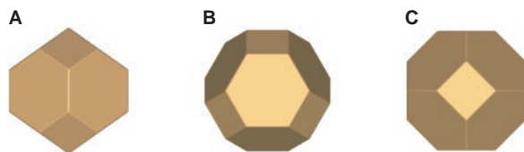
Fig. 3. Wigner-Seitz elementary cell of bcc tungsten. (A) View parallel to a \langle 110 \rangle crystal direction, showing a twofold symmetry with respect to a rotation around the vertical axis. (B) View parallel to a \langle 111 \rangle crystal direction with a threefold symmetry. (C) View parallel to a \langle 001 \rangle crystal direction displaying a fourfold symmetry.
