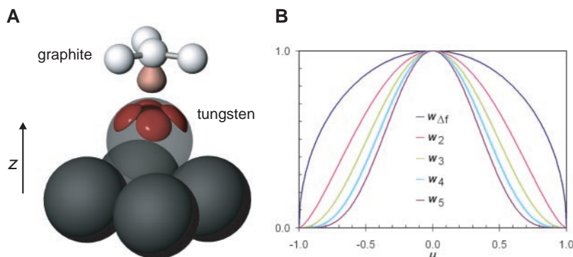
Fig. 1. (A) Front section of an idealized tungsten AFM/STM tip with part of a graphite sample on top. The tip consists of bulk W (001) with a bcc crystal structure. In this structure, one atom in the center of a cube is surrounded by eight atoms in the corners of the cube. The front atom of the tip corresponds to an adatom on W (001). The adatom has four local maxima in the charge density ( 4, 5 ). (B) Weight functions w_{\Delta f} and w_2 to w_5 (13). The frequency shift is given by a convolution of w_{\Delta f} with the derivative of F_{ts} with respect to z , and the n th harmonic a_n is given by a convolution of w_n with the n th derivative of F_{ts} with respect to z (13) (Eq. 1).
