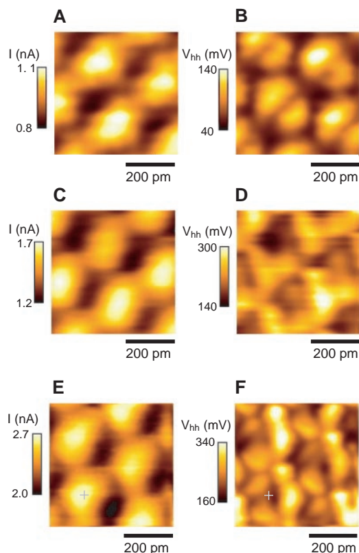
Fig. 2. Constant height measurement of tunneling current I (left column) and amplitudes of higher harmonics V_{hh} (right column). Typical acquisition time is 30 min per data set. The W tip was biased at a voltage of +100 mV with respect to the graphite sample and the fundamental oscillation amplitude was A = 300 pm. (A) Tunneling current for a tungsten state showing twofold symmetry in V_{hh} signal. Scanning speed, 1.25 nm/s. (B) V_{hh} signal, simultaneously recorded with (A). (C) Tunneling current for a tungsten state showing threefold symmetry in the V_{hh} signal. Scanning speed, 200 pm/s. (D) V_{hh} signal, simultaneously recorded with (C). (E) Tunneling current for a tungsten state showing fourfold symmetry in the V_{hh} signal. Scanning speed, 200 pm/s. (F) V_{hh} signal, simultaneously recorded with (E). The V_{hh} signal shows a four-leaf clover, centered close to the maximum of the current image (gray crosses) (Fig. 4). The symmetry of the V_{hh} signals in the right column points to the bonding symmetry of the W tip atom, as shown in Fig. 3.
