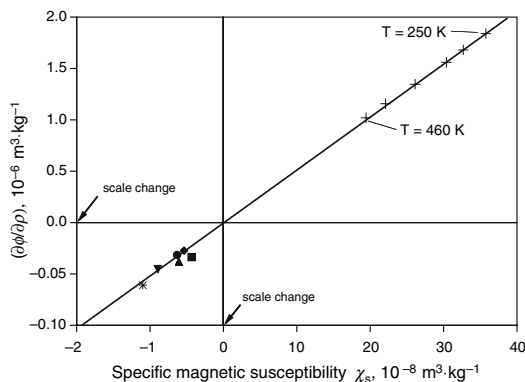
Fig. 4. Slope of the coupling factor (\partial\phi/\partial\rho) as a function of the specific magnetic susceptibility \chi_s of the fluid: ● helium; ■ neon; ◆ nitrogen; ▲ argon; * propane; ▼ toluene; + air at T=(250 to 460) K; — linear fit of the data.
