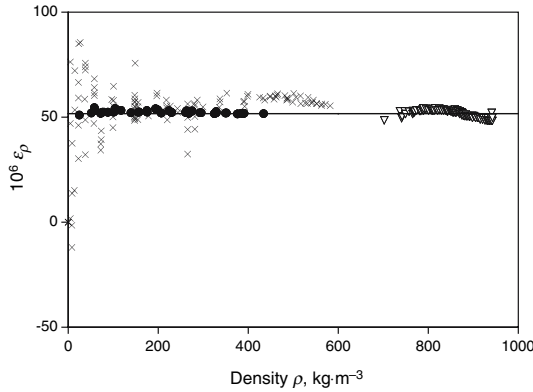
Fig. 5. Apparatus constant \epsilon_\rho for the fluid-specific effect for several fluids: \times propane; \nabla toluene; \bullet air; — \epsilon_\rho = 51.7 \times 10^{-6} determined from the two-sinker analysis.
