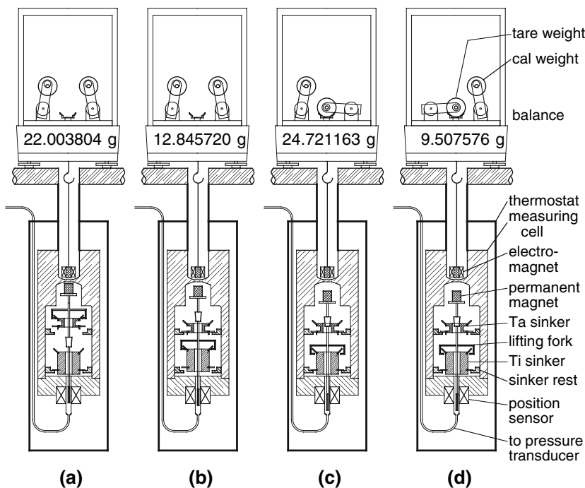
Fig. 1. Schematic of the two-sinker densimeter showing the four weighings; (a) weighing of the tantalum sinker, (b) weighing of the titanium sinker, (c) weighing of the balance calibration weight, and (d) weighing of the balance tare weight; in (c) and (d) both sinkers are on their rests. Balance displays are typical for a fluid density of 941 \text{ kg} \cdot \text{m}^{-3} . Figure is not to scale.
