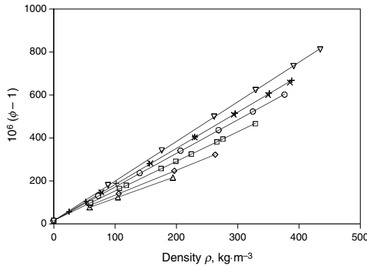
Fig. 3. Coupling factor \phi as a function of density \rho for air measured in the two-sinker densimeter at various temperatures and at pressures up to 38 MPa: \nabla 250 K; * 273 K (2 series); \circ 293 K; \square 340 K; \diamond 400 K; \triangle 460 K; — linear fits of the data at the various temperatures.
