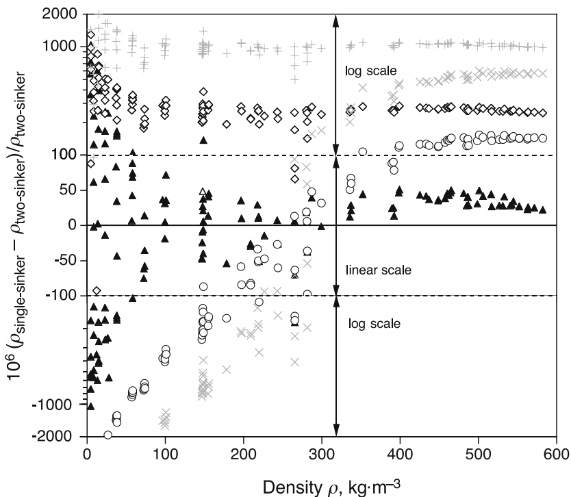
Fig. 6. Comparison of propane densities analyzed as single-sinker data with different corrections for the force transmission error: Ta sinker: \times no corrections ( \phi=1 ), + apparatus correction only ( \phi=\phi_0 ); Ti sinker: \circ no corrections ( \phi=1 ), \diamond apparatus correction only ( \phi=\phi_0 ); \blacktriangle including fluid effects (Eq. (26)).
