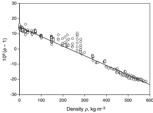
Fig. 2. Coupling factor \phi as a function of density \rho for propane measured in the two-sinker densimeter: \circ data; — linear fit of the data.
