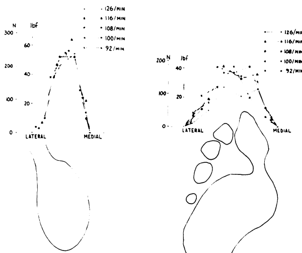
FIG. 8 FIG. 9 The distribution of peak loads across the heel (Fig. 8) and the forefoot (Fig. 9) in the same subject at walking speeds from ninety-two to 126 paces per minute. The heel shows a similar pattern at all walking speeds. The forefoot distributes the load more to the lateral side of the foot at the slowest walking rate.
