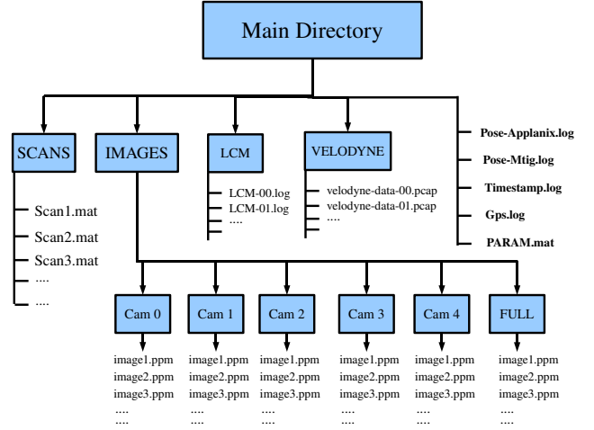
Fig. 3. The directory structure containing the data set. The rectangular blocks represent folders.
