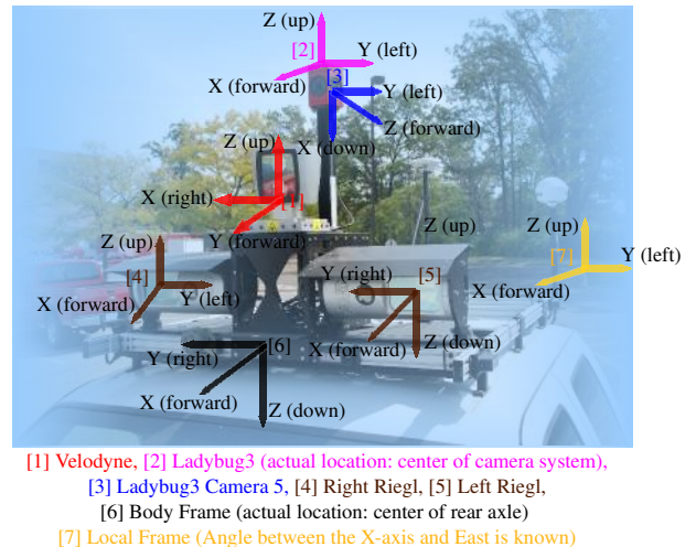
Fig. 2. Relative position of the sensors with respect to the body frame.
