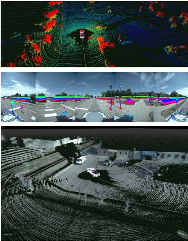
Fig. 7. The top panel is a perspective view of the Velodyne lidar range data, color-coded by height above the estimated ground plane. The center panel shows the above-ground-plane range data projected into the corresponding image from the Ladybug3 cameras. The bottom panel shows the Screenshot of the viewer showing the RGB textured point cloud corresponding to a parking lot in downtown Dearborn captured during one of the trials in the month of December.
