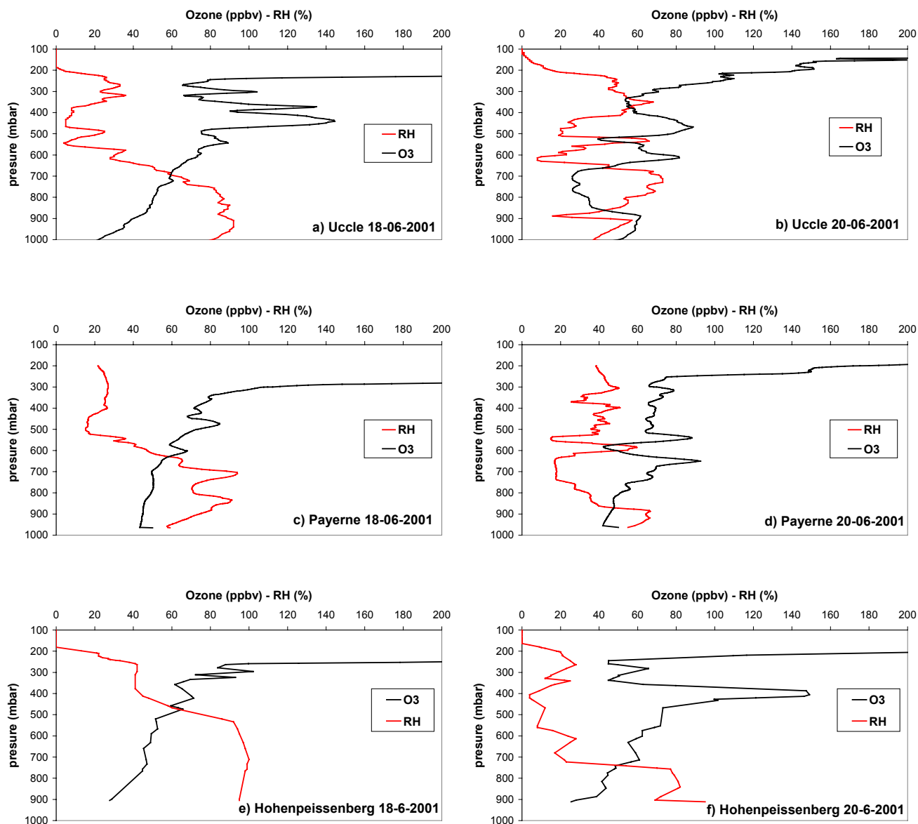
Fig. 5. Profile measurements of ozone and RH based on ozonesonde launches on 18 and 20 June 2001 at Uccle (a and b) at 11:00 UTC, at Payerne (c and d) at 11:00 UTC and at Hohenpeißenberg (e and f) at 05:00 UTC.
