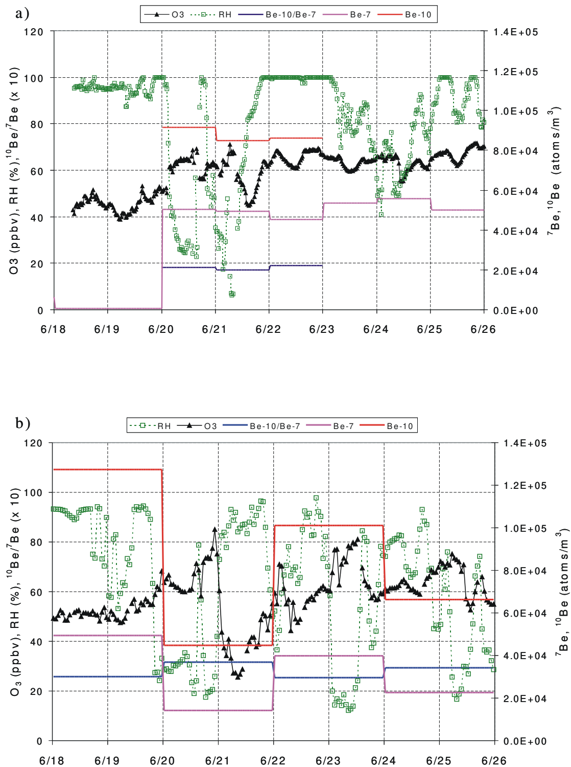
Fig. 7. Surface measurements of RH, ozone, {}^7\text{Be} , {}^{10}\text{Be} concentrations and their ratio {}^{10}\text{Be}/{}^7\text{Be} at Zugspitze (a) and at Jungfraujoch (b), during the period 18–25 June 2001; the time is CET. The {}^7\text{Be} , {}^{10}\text{Be} concentrations and their ratio are daily values at Zugspitze and bi-daily at Jungfraujoch.
