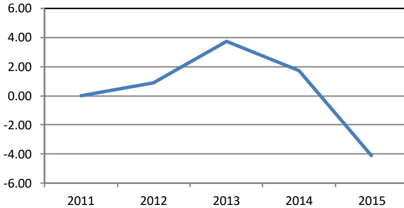
Fig. 2. FVA_{1,t} : stage 1 vs. naive-placebo. Source: author's elaboration
