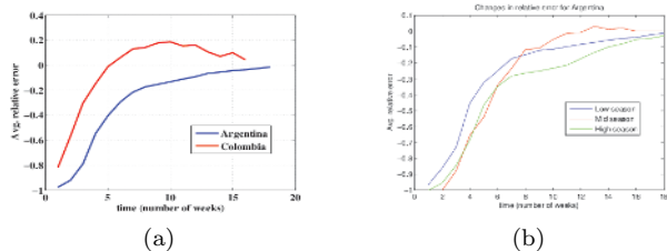
Figure 2: Average relative error of PAHO count values with respect to stable values. (a) Comparison between Argentina and Colombia (b) Comparison between different seasons for Argentina.
