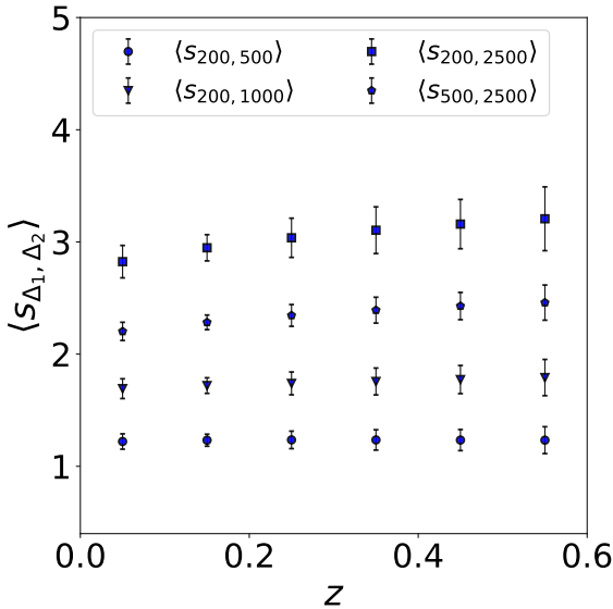
Figure 8. Synthetic average sparsity data \langle s_{200,500} \rangle (circles), \langle s_{200,1000} \rangle (triangles), \langle s_{200,2500} \rangle (squares) and \langle s_{500,2500} \rangle (pentagons). The error bars indicate the amplitude of statistical errors due to the propagation of mass measurement uncertainties.
