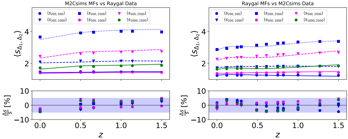
Figure A2. Left panel: average halo sparsity for different overdensity configurations as a function of redshift predicted by solving Eq. (3) using the M2Csims calibrated multiplicity functions for the Raygal cosmology plotted against the average sparsities from the Raygal halo catalogues. Right panel: average halo sparsities predicted by solving Eq. (3) using the Raygal calibrated multiplicity functions for the M2Csims cosmology plotted against the average sparsities from the M2Csims halo catalogues. The lower panels show the relative difference between the predictions and the N-body halo catalogue estimates.
