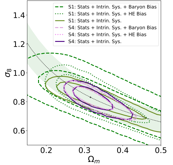
Figure 9. 1 and 2\sigma credibility regions in the \Omega_m - \sigma_8 plane from the analysis of the synthetic dataset with different error assumptions for the S1 and S4 cases respectively. The best-fit values of \Omega_m and \sigma_8 from the different parameter inferences coincide with the values of the fiducial cosmology marked by the cross-point. The dashed line and the green shaded area corresponds to curves of constant S_8 = 0.852 \pm 0.104 values, that is the mean and standard deviation of S_8 from the MCMC chains of S1 case with intrinsic systematic errors and baryon bias. We can see that using multiple sparsity estimates breaks the S_8 degeneracy.
