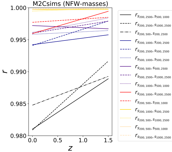
Figure 4. Sparsity correlation coefficients obtained using the mass estimates from the best-fit NFW profiles of the M2Csims halo catalogues. As we can see, contrary to the correlations among sparsities estimated from the SO halo masses, assuming that the density profile of haloes is described by NFW profile artificially correlates sparsities to order r \approx 1 , even those probing mass distribution in mass shells at large separations.
