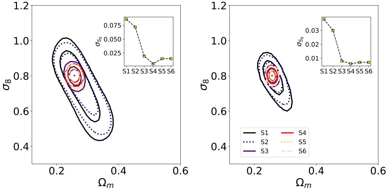
Figure 5. 1 and 2\sigma credibility contours in the \Omega_m - \sigma_8 plane for the Raygal synthetic datasets. The different lines correspond to the sparsity configurations S1-S6 described in Section 3.1 assuming statistical errors on the average sparsity estimates of \sigma_{(s(z))} = 0.3 (left panel) and \sigma_{(s(z))} = 0.1 (right panel). The cross corresponds to the cosmological parameter values of the fiducial Raygal cosmology. As the best-fit parameters for the different sparsity configurations coincide with those of the fiducial model, we do not show them in the plot to avoid cluttering. The inset plot shows the 1\sigma error on \sigma_8 as a function of the number of average sparsity configurations S1-S6. As we can see the uncertainties saturate beyond S4.
