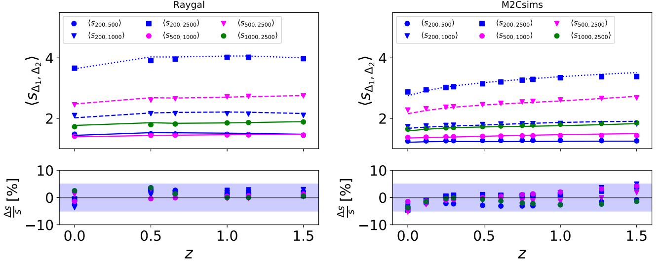
Figure 2. Average halo sparsity estimates for different overdensity configurations as a function of redshift for the Raygal (left panel) and M2Csims (right panel) halo catalogues. The data points in the plots correspond to the N-body estimates, while the various lines show the analytical predictions from the average sparsity relation of Eq. (3) that has been solved using the ST-parametrised mass functions calibrated on the simulations. The relative differences between the N-body and analytical results are shown in the bottom panels, where the shaded areas delimit the regions with less than 5 per cent relative differences. Differences between the average sparsity values from the Raygal and M2Csims halo catalogues for the same overdensity pairs pertain to the differences of the simulated cosmological models.
