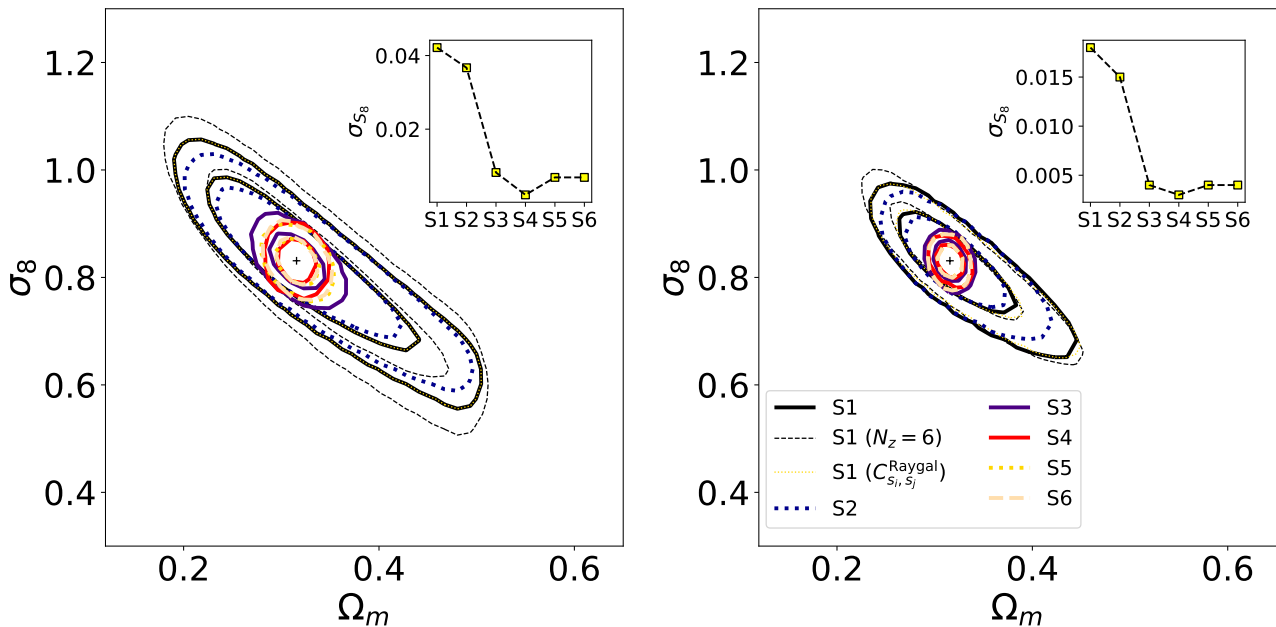
Figure 6. As in Fig. 5 but for the M2Csims case. In addition to the sparsity combinations S1-S6, we also show the 1 and 2\sigma contours for the S1 case with N_z = 6 redshift bins in the redshift interval 0 < z < 1.5 (thin black dashed lines) rather than the nominal N_z = 11 (black solid line), and with covariance from the Raygal simulation (yellow dotted line).
