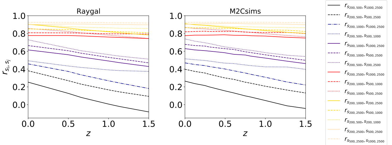
Figure 3. Sparsity correlation coefficients from the Raygal (left panel) and M2Csims (right panel) halo catalogues, respectively. As we can see over the redshift range 0 < z < 1.5 , sparsity combinations probing the halo mass distribution in close (overlapping) mass shells are highly correlated ( r \gtrsim 0.5 ). This is not the case of sparsities associated to mass shells that are at larger separations ( r \lesssim 0.5 ).
