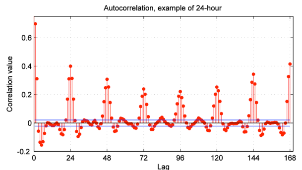
Figure 2 - Autocorrelation example, when data best correlates at 24 hour intervals.
