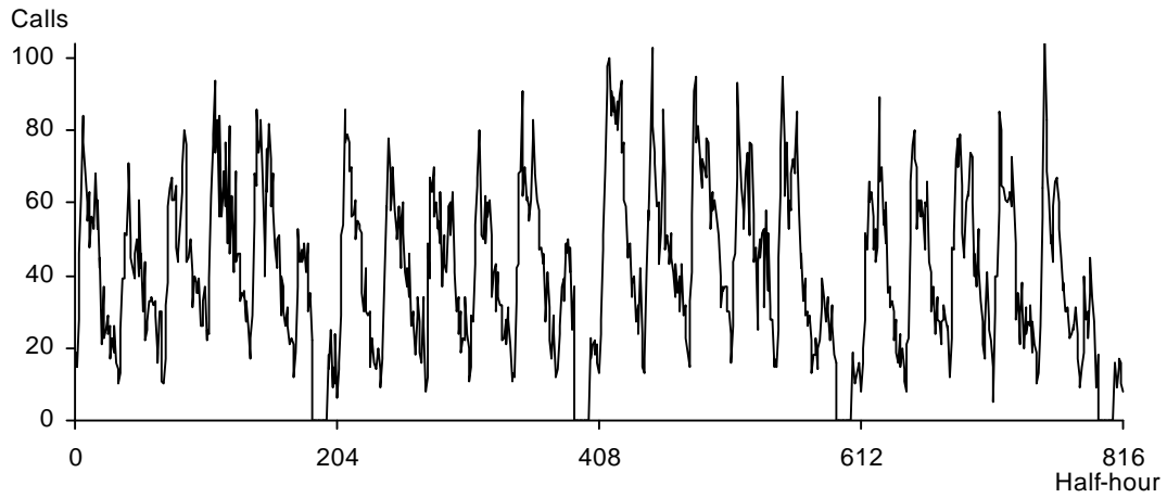
Fig. 5. Half-hourly arrivals at the Israeli bank call centre for the four-week period from Sunday 28 November to Saturday 25 December 1999. ‘Manipulated’ arrivals series is plotted. In this series, each weekend is presented as one day, and each week consists of 6 \times 34 = 204 half-hourly periods.
