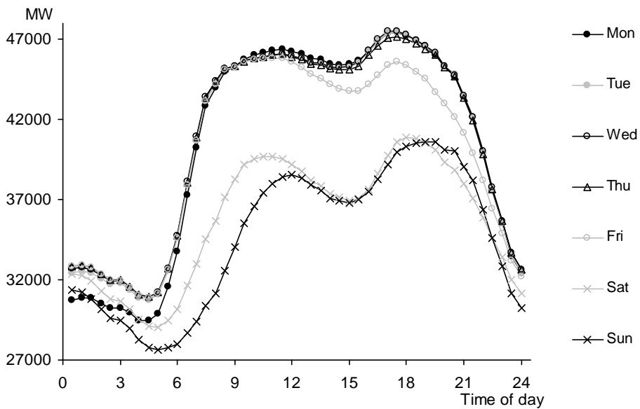
Fig. 2. Average intraday cycle for each day of the week for the British load data. Calculated using the two-year estimation sample.
