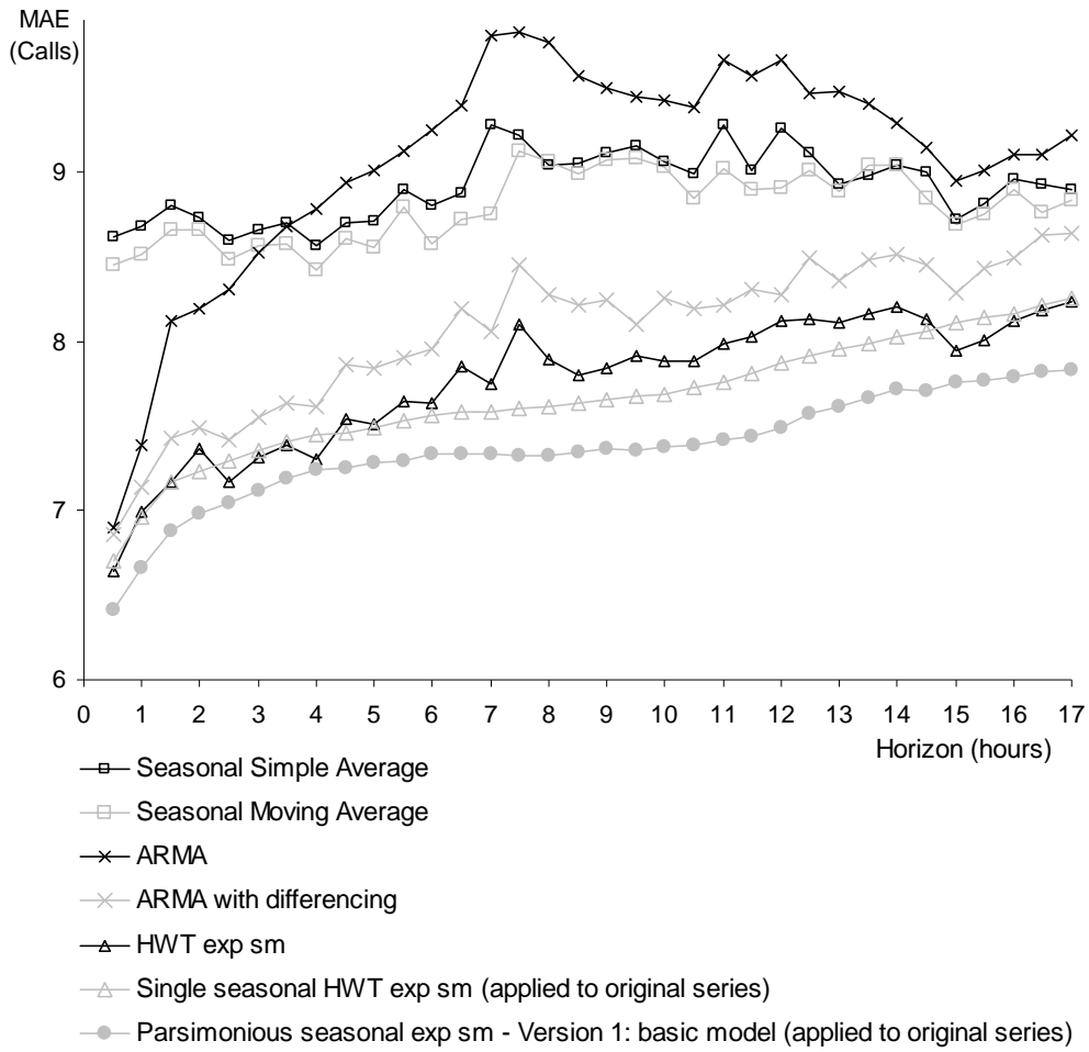
Fig. 7. Post-sample MAE for the Israeli bank call centre series. Two methods were applied to the original arrivals series, and the rest to the ‘manipulated’ arrivals series.
