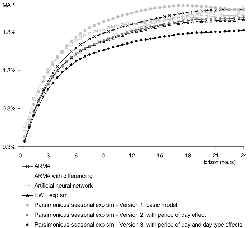
Fig. 4. Average post-sample MAPE for the British and French load series.
