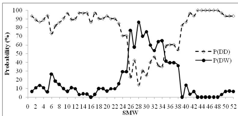
Fig. 4: Conditional probability of dry/dry and dry/wet spell
