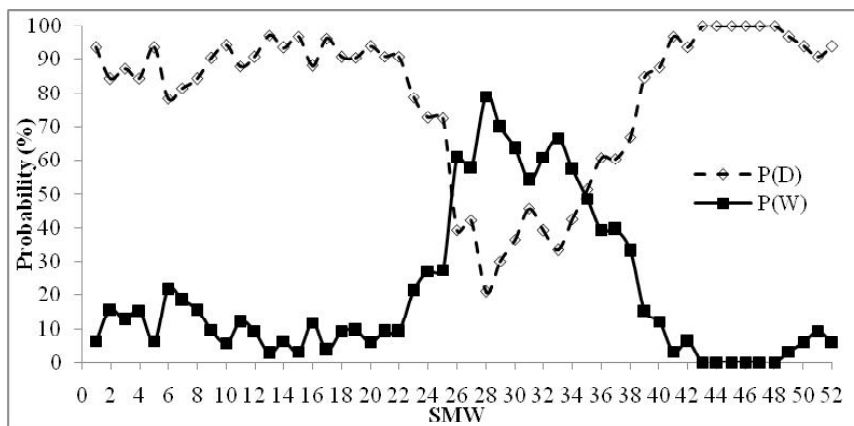
Fig. 3: Initial probability of dry spell and wet spell
