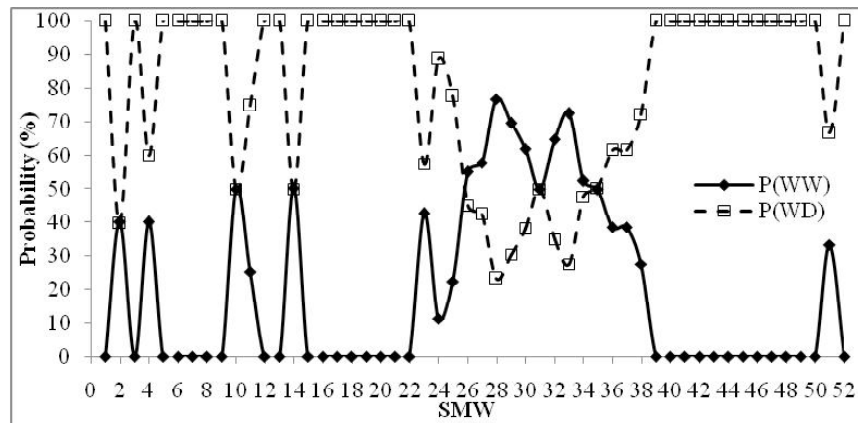
Fig. 5: Conditional probability of wet/dry and wet/wet spell
