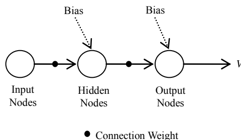
Figure 3. Nonlinear autoregressive network (NAR).
