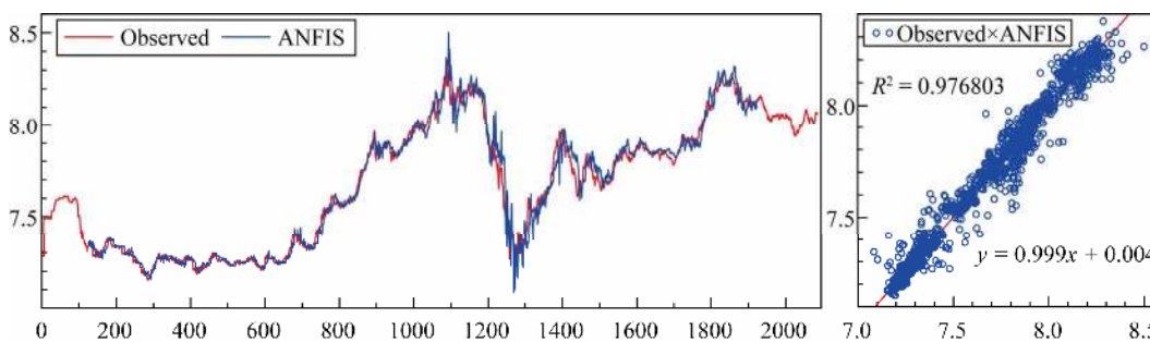
Figure 8. Depicted graph and scatter plots for the observed and ANFIS prediction.
