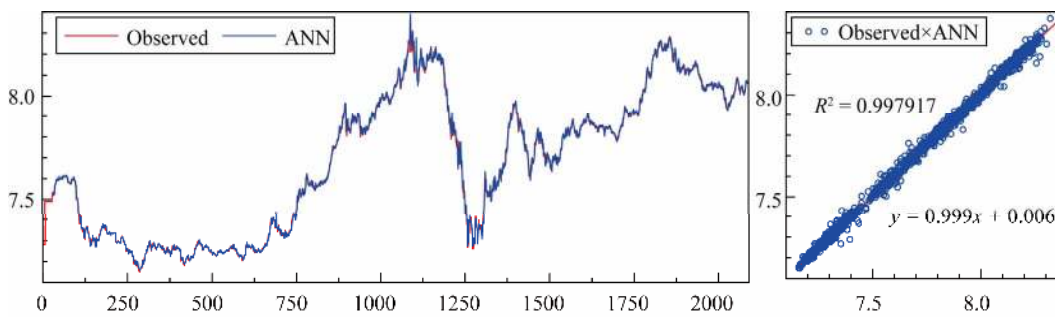
Figure 7. Depicted graph and scatter plots for the observed and ANN prediction.
