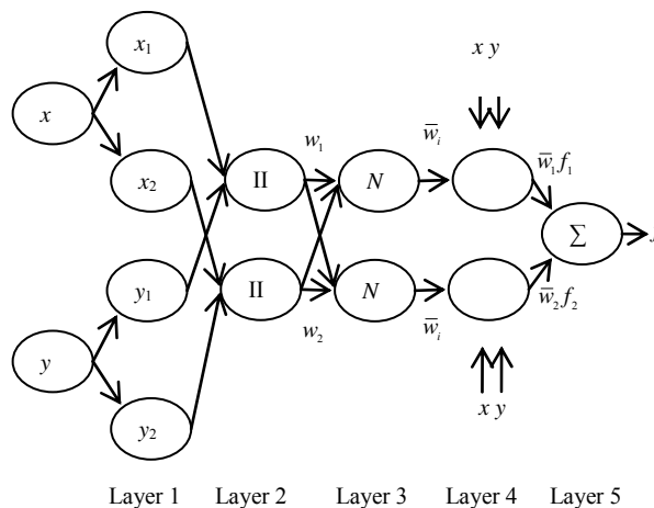
Figure 4. The basic architecture of the ANFIS model.
