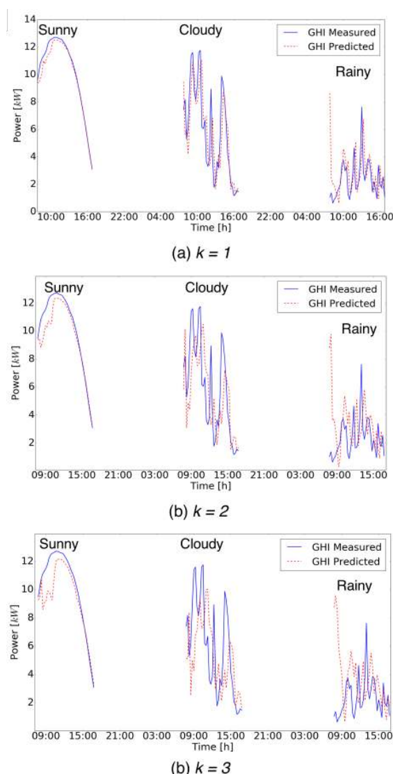
Figure 6: Simulations of PV energy production with k = 1 and k = 2 (June 2013)
