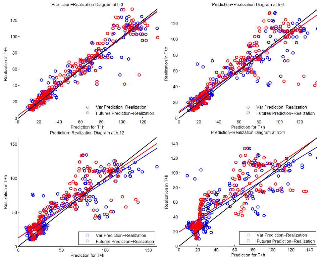
Figure 1. Prediction-Realization Diagrams for VAR and Futures Forecasts
