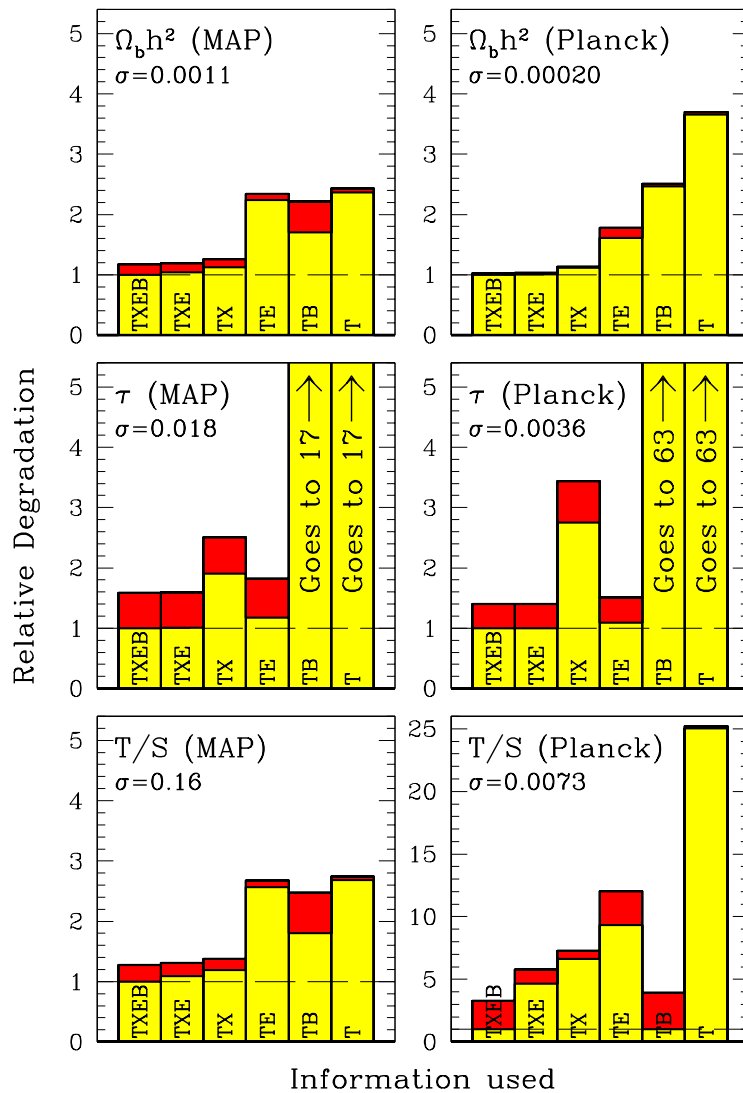
FIG. 25.—Information about cosmological parameters from different polarization types. In each panel, the bars show the relative error bars using all information ( TXEB ), all but B -polarization ( TXE ), T and X only ( TX ), T and E only ( TE ), and unpolarized intensity alone ( T ). Results are shown both without any foregrounds (light shaded region) and for the MID foreground scenario with known properties (dark shaded region). Note that this figure uses a Gaussian rather than exponential coherence function. The rightmost bars in the \tau panels extend far off the scale.
