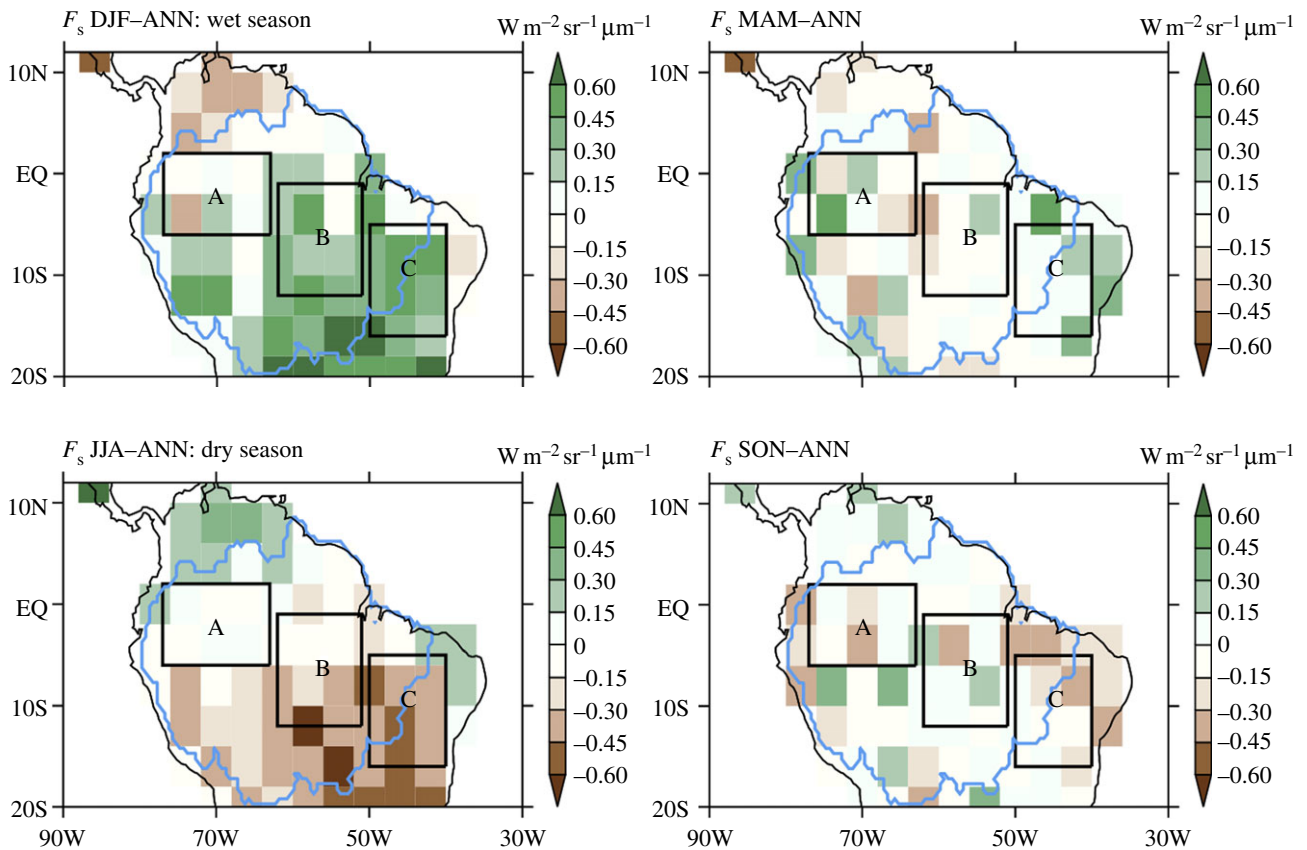
Figure 1. Seasonal variation of chlorophyll fluorescence, F_s ( \text{W m}^{-2} \text{sr}^{-1} \mu\text{m}^{-1} ), retrieved from GOSAT in 755 nm over Amazonia during June 2009–May 2010. The annual mean is subtracted from the seasonal mean to show fluorescence seasonality. Boxes A, B and C are relative everwet, wet and dry areas, respectively, for the analysis in figures 2 and 3. The outline in the map line represents the Amazon basin. The resolution in the figure is coarse because GOSAT provides only one measurement at every 4 s and the retrieval exhibits a high single measurement noise. (Online version in colour.)
