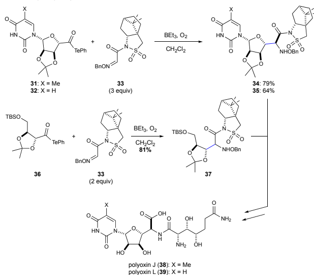
Scheme 9. Key steps in the synthesis of polyoxins J (38) and L (39) by Inoue and coworkers.
