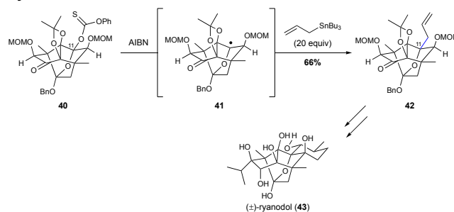
Scheme 10. Key step in the synthesis of ryanodol (43) by Inoue and coworkers.
