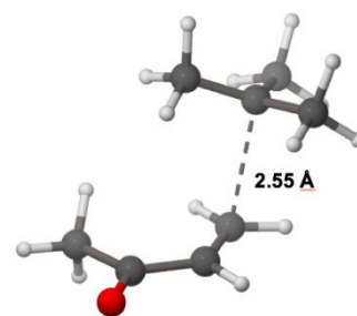
Figure 1. The long forming-bond in the transition state for the addition of a nucleophilic tertiary carbon
