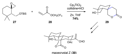
Scheme 8. Reisman's synthesis of maeocrystal Z (30) from Giese coupling of a tertiary radical formed by Ti-promoted reductive opening of an epoxide
