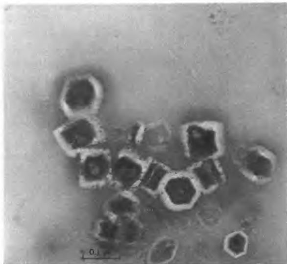
FIGURE 12.—Electron photomicrograph of microcrystalline gibbsite.
