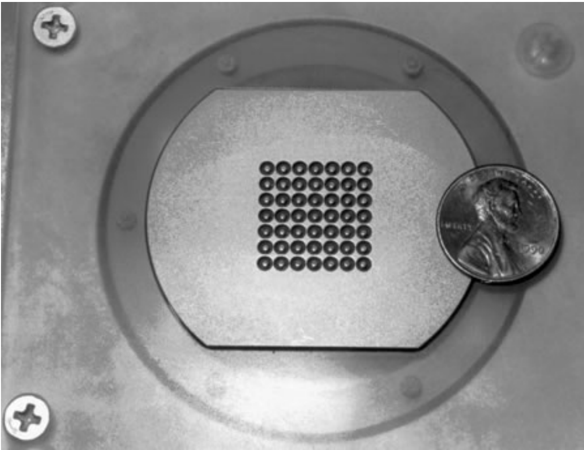
Figure 1. Photograph of a 7×7 array of stainless-steel electrodes, 2.54 mm apart. A U.S. penny is shown for size comparison.
