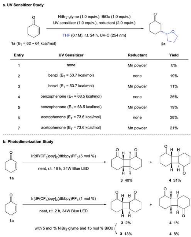
Scheme 2 Mechanistic studies.
