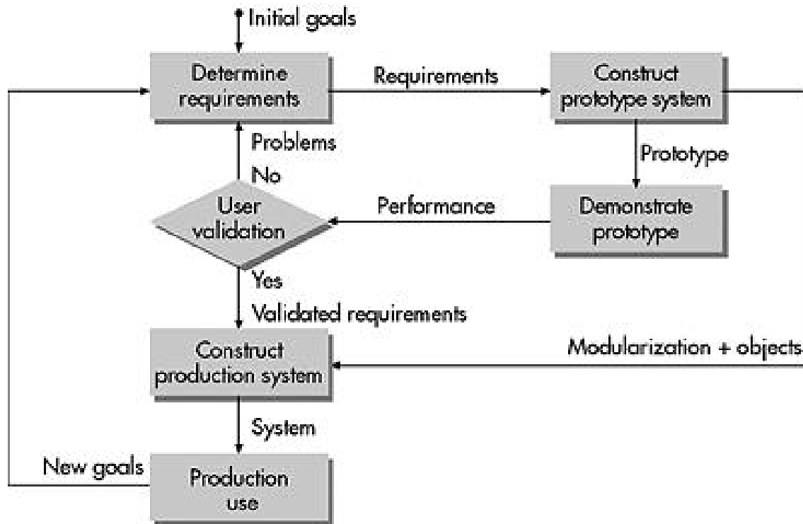
Figure 1. An iterative prototyping life cycle. Once constructed, the prototype is demonstrated to check its actual behavior against its expected behavior. This helps identify problems and can lead to a redefinition of requirements.
