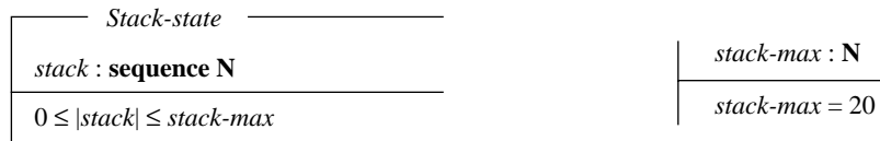
Fig. 20 The state space of a simple stack in Z.
