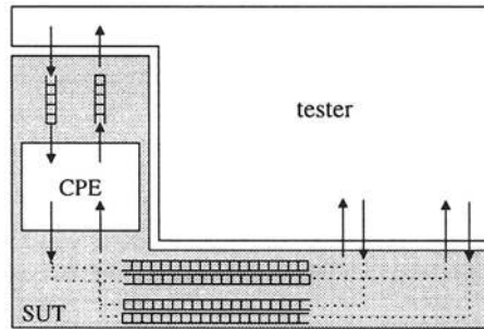
Figure 4 Formal model of the SUT
