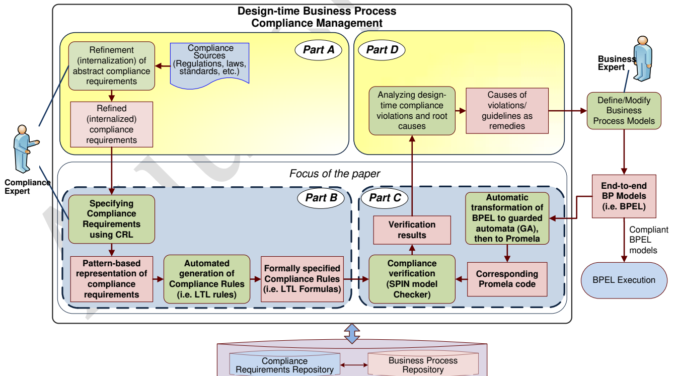
Fig. 1. Design-time business process compliance management approach.
