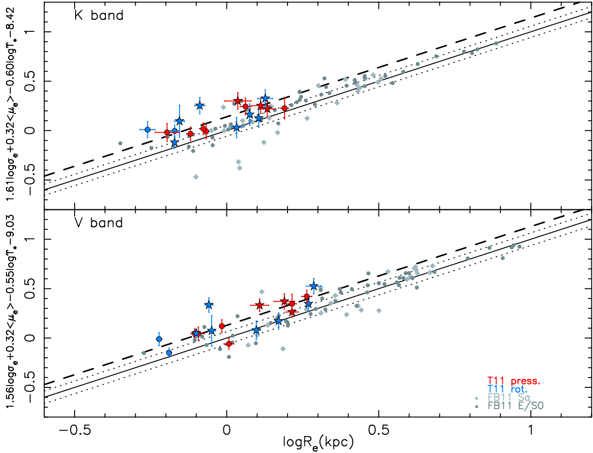
Fig. 6. Fundamental plane in the K and V bands when the stellar mass-to-light ratio ( \Upsilon_* ) is included. Symbols as in Fig. 2.
