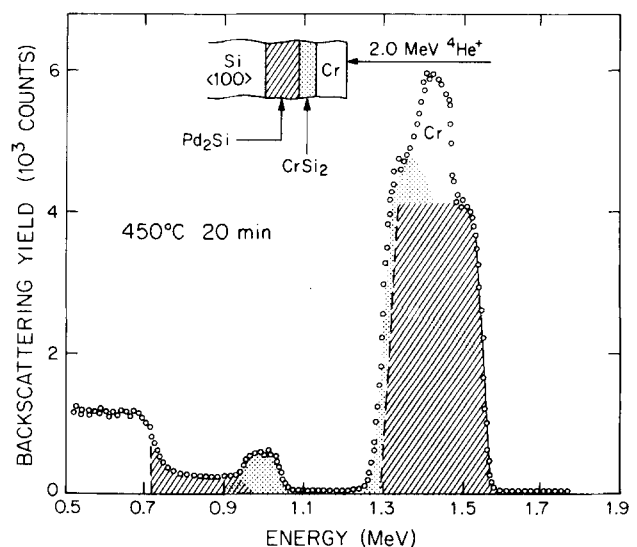
FIG. 6. ^4\text{He}^+ backscattering spectrum of Pd (1400 Å) and Cr (1200 Å) evaporated in that order on a Si \langle 100 \rangle single crystal and annealed at 450°C for 20 min. All Pd has reacted with Si to form \text{Pd}_2\text{Si} before \text{CrSi}_2 was formed on top.
