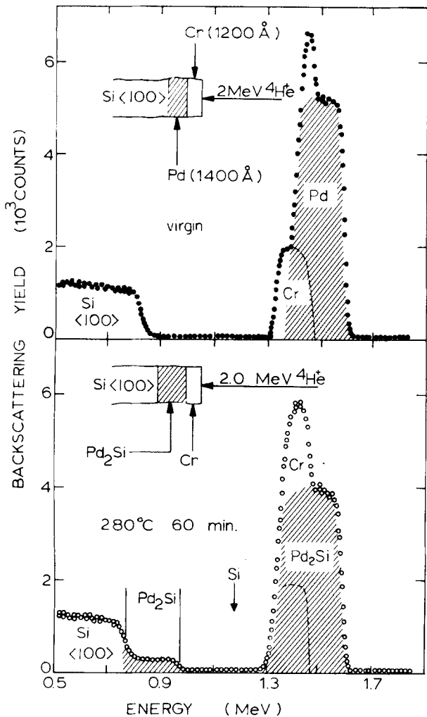
FIG. 5. ^4\text{He}^+ backscattering spectrum of Pd (1400 Å) and Cr (1200 Å) evaporated in that order on Si \langle 100 \rangle single crystal before (top) and after (bottom) annealing at 280°C for 60 min. The reaction between Pd and Si results in the formation of \text{Pd}_2\text{Si} , while there is no apparent interaction between Pd and Cr.
