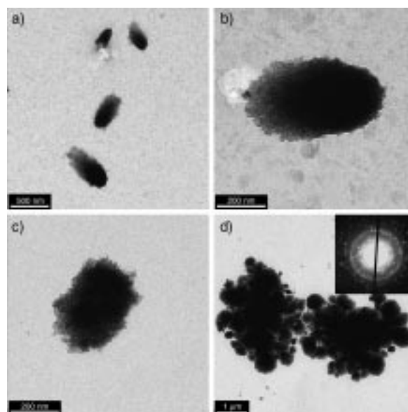
Figure 6. BaSO 4 particles obtained in the presence of PEG- b -PMAA-PO 3 H 2 with an ageing time of 1 h: a, b) in glass tubes, and c) on carbon films. d) shows particles obtained after an ageing time of 3 h. Inset of d) shows the corresponding electron diffraction pattern that exhibits sharp spots corresponding to the barite structure.
