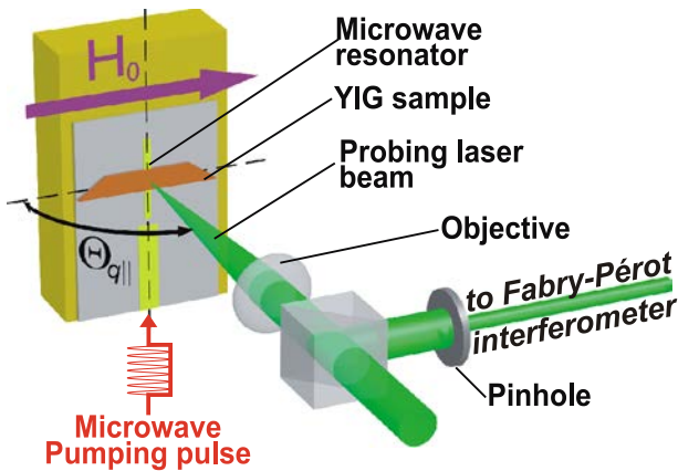
Fig. 2. (Color online) Geometry of the experiment. The setup allows to vary the probing laser beam incidence angle \Theta_{q\parallel} allowing for wavevector resolution. The YIG sample is placed on top of a microstrip resonator which is fabricated on top of an alumina substrate. Microwave pumping pulses are applied to the microstrip in order to drive the spin-wave system. The probing laser beam is directed through a beam splitter and focused by objective on to the YIG sample. The inelastically scattered light is redirected to the Fabry–Pérot interferometer. An additional pinhole is used to increase the wavenumber resolution.
