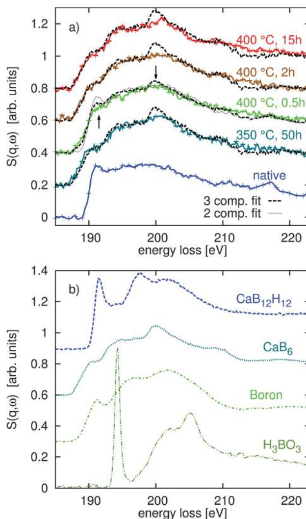
Fig. 3 (a) XRS spectra of the B K-edge for the native \text{Ca}(\text{BH}_4)_2 sample and the sample after decomposition at different temperatures and annealing durations. The component fits are shown as dashed black lines (combination of \text{CaB}_6 , B, and \text{Ca}(\text{BH}_4)_2 ), a thin grey line represents the results from a linear combination of reference spectra (B and \text{Ca}(\text{BH}_4)_2 ) according to the fit results of the Ca L_{2,3} -edges and the subsequent estimation of the boron containing phases. (b) XRS spectra of the B K-edge of the reference compounds \text{CaB}_{12}\text{H}_{12} , \text{CaB}_6 , B, and \text{H}_3\text{BO}_3 . As the Ca L_{2,3} -edges, the B K-edge shows distinctly different shapes and different features for the different reference compounds.
